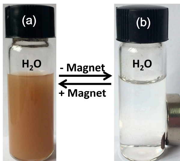
Figure S2. Photographs of the dispersion-collection process of \text{Fe}_3\text{O}_4@1 in water.
