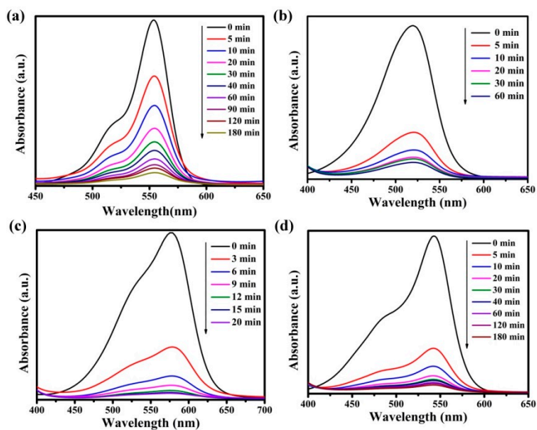
Figure S4. Adsorption spectra of the RhB solution (a); the T solution (b); the GV solution (c) and the FB solution (d) under the dark in presence of \text{Fe}_3\text{O}_4@1 .
