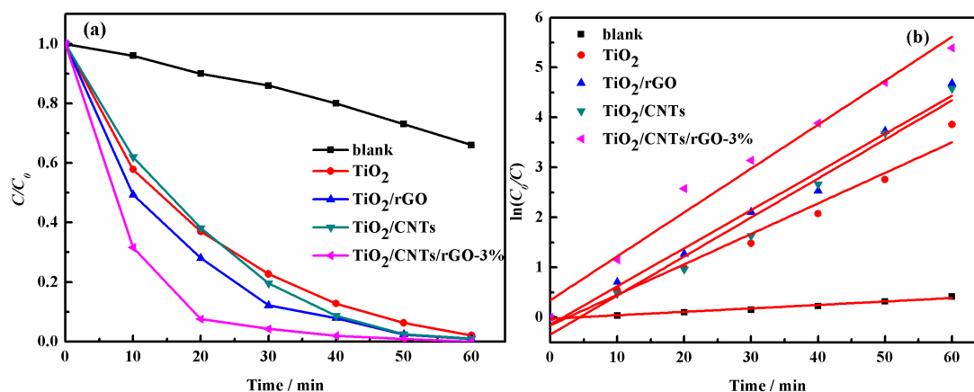
Figure 4. Blank test, TiO_2 , TiO_2/rGO , TiO_2/CNTs and TiO_2/CNTs/rGO-3\% : (a) plot of C/C_0 vs. irradiation time of RhB degradation; (b) linear transform \ln(C_0/C) = kt of the kinetic curves of RhB degradation.
