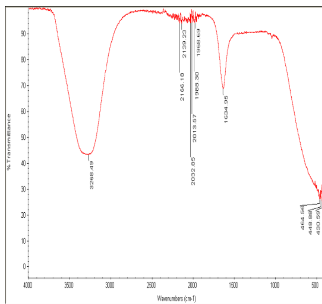
FTIR spectra synthesized silver nanoparticle by Ferula asafetida alcoholic extract
