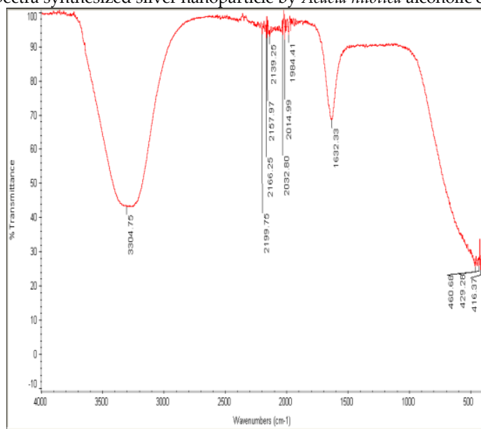
FTIR spectra synthesized silver nanoparticle by Acacia nilotica aqueous extract
