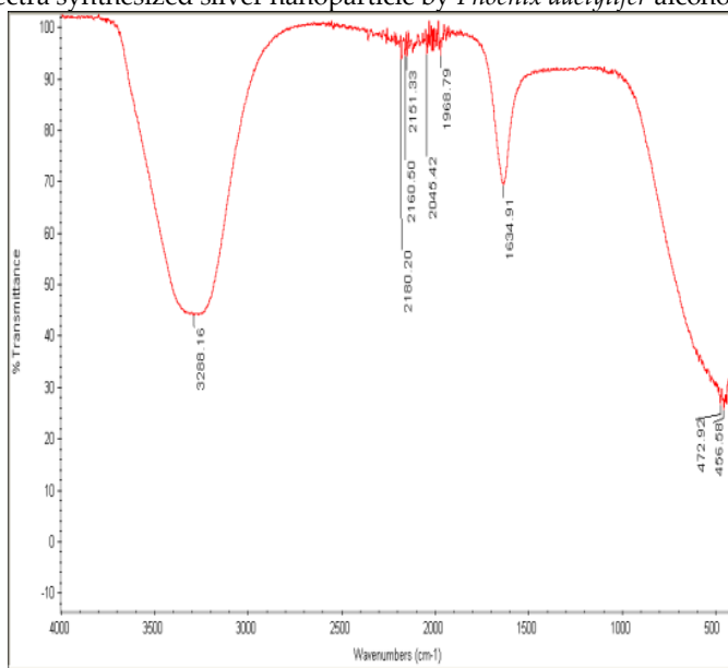
FTIR spectra synthesized silver nanoparticle by Phoenix dactylifer aqueous extract
