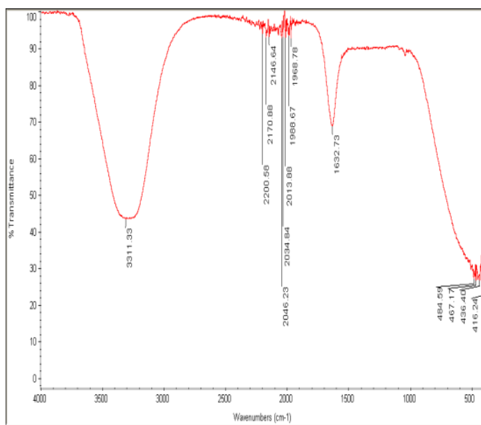
FTIR spectra synthesized silver nanoparticle by Acacia nilotica alcoholic extract
