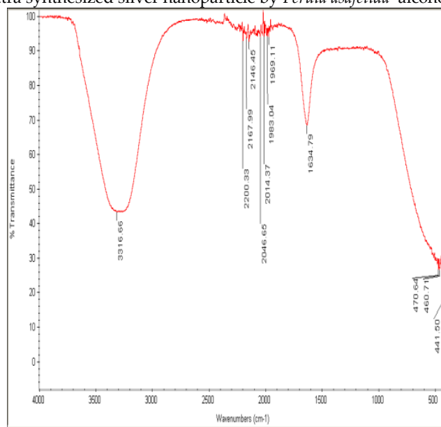
FTIR spectra synthesized silver nanoparticle by Ferula asafetida aqueous extract
