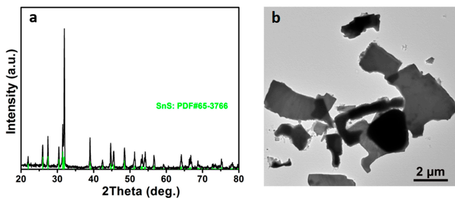
Figure S2. (a) XRD pattern and (b) TEM image of SnS nanoplates.
