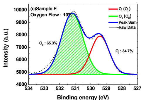
Figure 6. XPS O 1s spectra of InTiZnO thin films with various oxygen flow ratios: (a) Sample A, (b) Sample B, (c) Sample C, (d) Sample D, and (e) Sample E.
