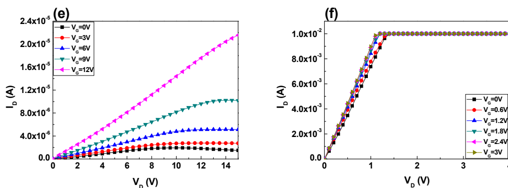
Figure 4. I_D - V_D of InTiZnO TFTs as a function of oxygen flow ratios: (a) Sample A, (b) Sample B, (c) Sample C, (d) Sample D, and (e) Sample E, and (f) Sample F with 0% oxygen flow ratio.
