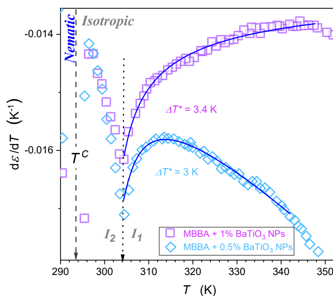
Figure 7. The focused insight for the behavior of dielectric constant in the isotropic liquid phase in MBBA-based nanocolloids for larger concentrations of nanoparticles. Solid curves are associated with the parameterization via Equation (5). Reference data are taken from Figure 4. The gray dashed arrow indicates the isotropic-nematic phase transition temperature T^C . Note: the transition occurs within the isotropic liquid phase, which suggests the liquid-liquid transition ( I_2 \leftarrow I_1 )—indicated by the dotted arrow.
