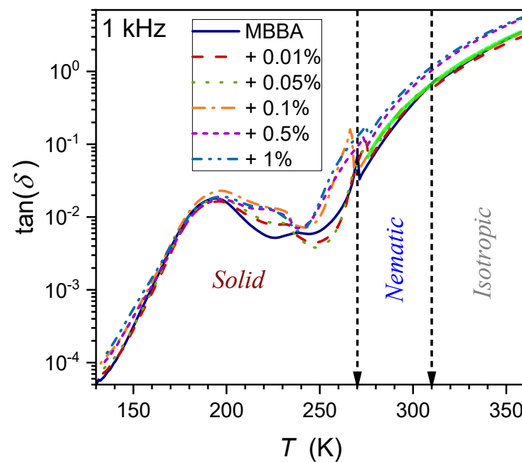
Figure 15. Temperature evolutions for tg\delta loss factor (frequency f = 1 kHz) in MBBA and related nanocolloids with BaTiO 3 nanoparticles. The solid green curve is related to Equation (18) with the exponent \phi \approx 2.8 .
