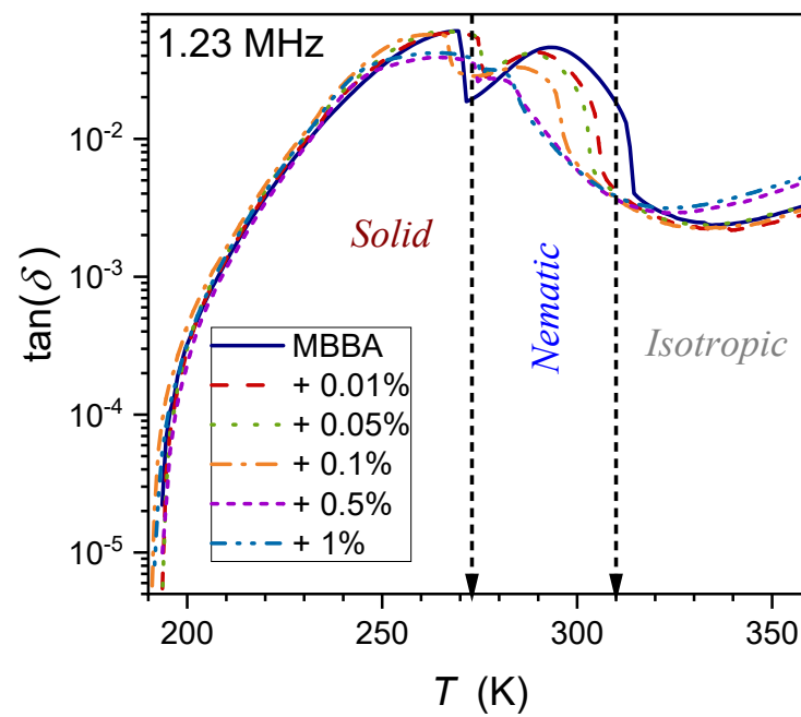
Figure 14. Temperature evolutions for tg\delta loss factor (frequency f = 1.23 MHz) in MBBA and related nanocolloids with BaTiO 3 nanoparticles.
