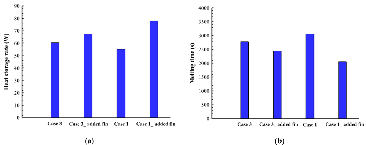
Figure 13. (a) Heat storage rate in Watt, (b) Melting time in seconds for cases 1, 3, 6, and 7 during the melting process.
