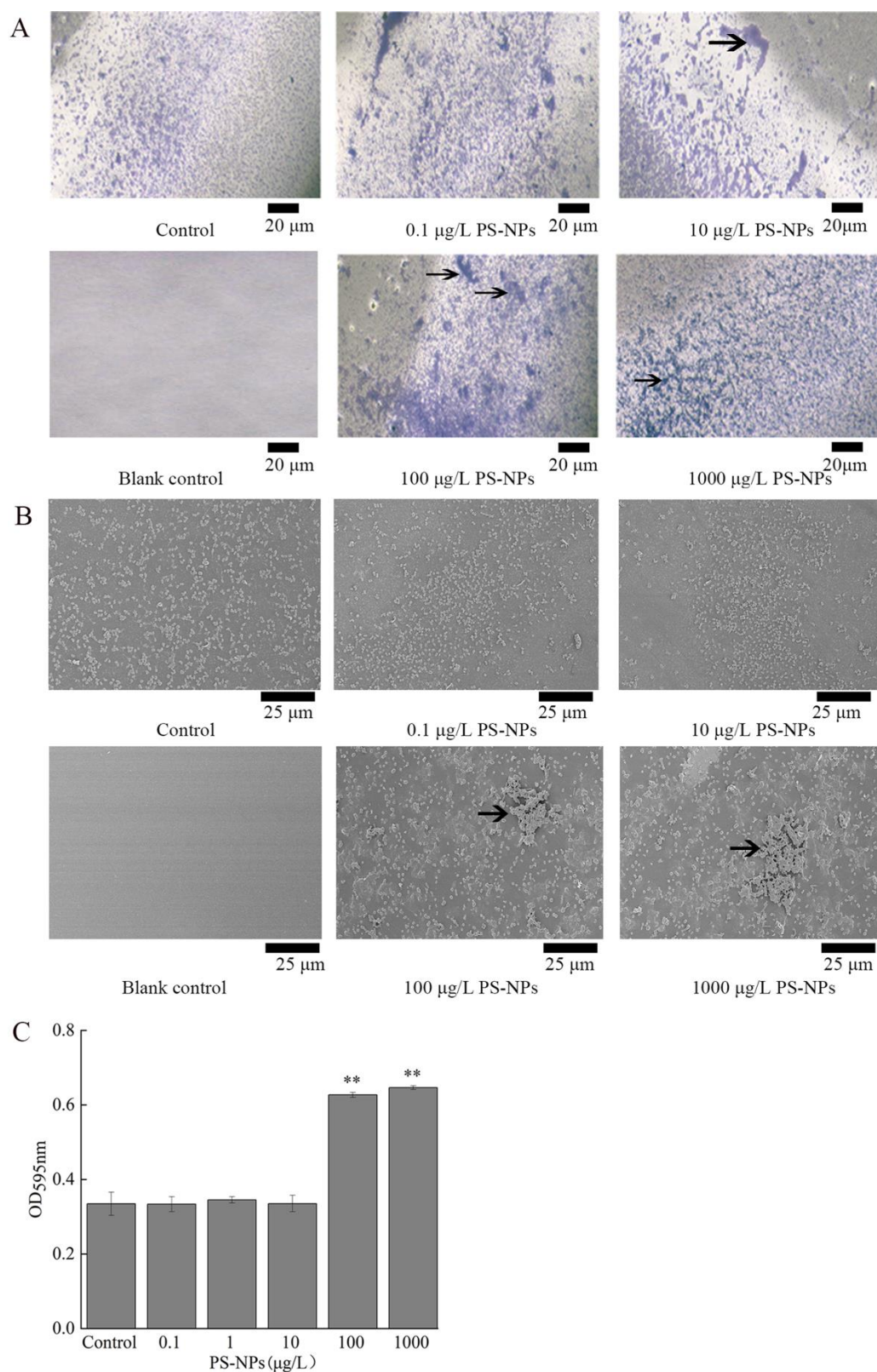
Figure 5. Effect of nanopolystyrene particle (NP) exposure at concentrations of 0.1–1000 µg/L on A. johnsonii AC15 biofilm formation. (A) Crystal violet staining images showing the effect of NP exposure at different concentrations on A. johnsonii AC15 biofilm formation. Arrowheads indicate the formed biofilm. (B) Scanning electron microscopy (SEM) images showing the effect of NP exposure at different concentrations on A. johnsonii AC15 biofilm formation. Arrowheads indicate the formed biofilm. (C) Effect of NP exposure at different concentrations on the amount of A. johnsonii AC15
