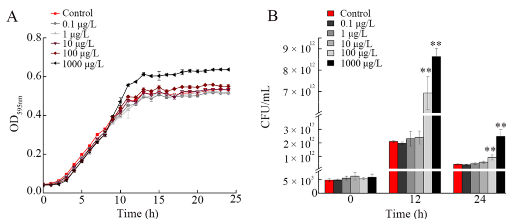
Figure 3. Effect of nanopolystyrene particle (NP) exposure on growth of A. johnsonii AC15. (A) Growth curves of A. johnsonii AC15 after exposure to NPs at different concentrations. (B) Effect of
