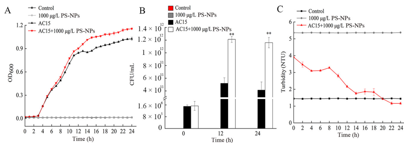
Figure 4. Adsorption curve of nanopolystyrene particles (NPs) during bacterial growth. (A) A. johnsonii AC15 growth curve after exposure to 1000 \mu\text{g/L} NP. (B) Effect of 1000 \mu\text{g/L} NP exposure on colony-forming unit (CFU) of A. johnsonii AC15 at different times. ** p < 0.01 vs. A. johnsonii AC15. (C) Turbidity analysis of bacterial solutions after cultivation at 37 °C for 24 h.
