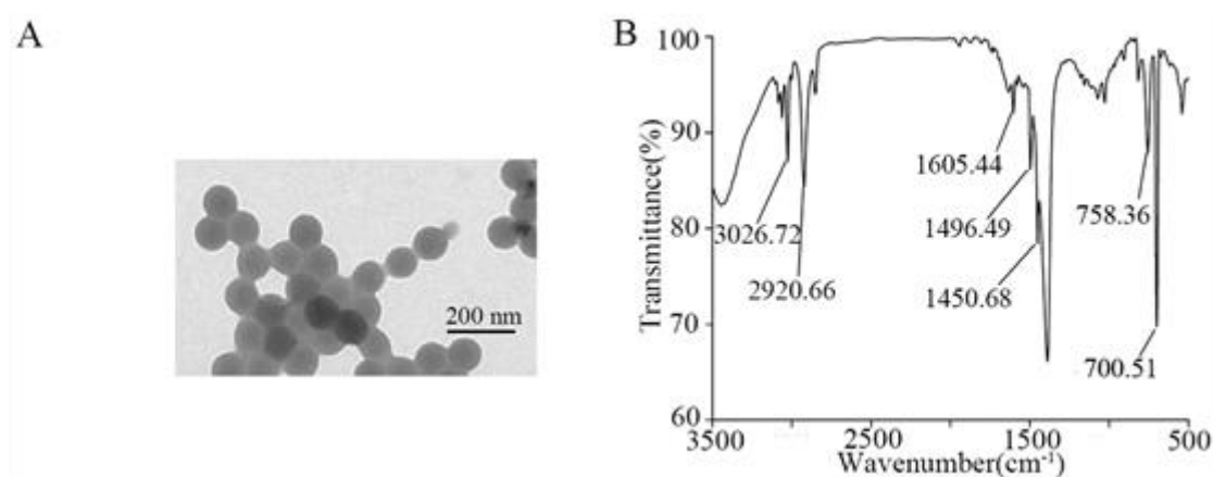
Figure 1. Nanopolystyrene particles (NPs) properties. (A) Transmission electron microscopy (TEM) image of NP suspension before the sonication. (B) FTIR spectrum of NPs.
