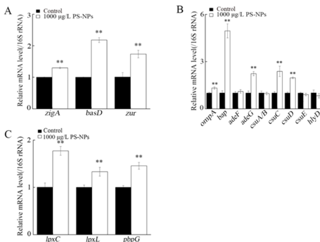
Figure 7. Effect of nanopolystyrene particle (NP) exposure on expression of virulence genes in A. johnsonii AC15. (A) Survival related genes. (B) Biofilm formation related genes. (C) Serum resistance related genes. ** p < 0.01 vs. Control.
