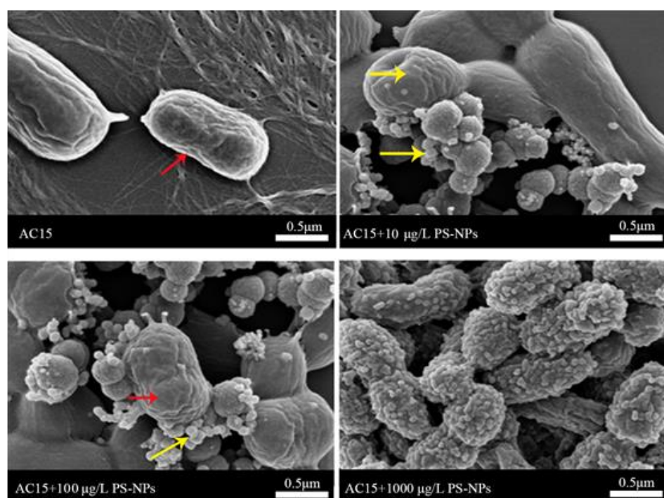
Figure 2. Scanning electron microscopy (SEM) images showing the aggregation of nanopolystyrene particle (NP) particles at concentrations of 10–1000 µg/L on surface of A. johnsonii AC15. Red arrowheads indicate A. johnsonii AC15. Yellow arrowheads indicate the aggregated NPs on surface of A. johnsonii AC15.
