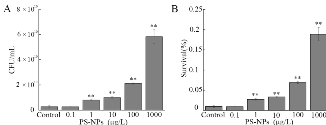
Figure 6. Effect of nanopolystyrene particle (NP) exposure on serum resistance of A. johnsonii AC15. (A) Colony-forming unit (CFU) of A. johnsonii AC15 in normal human serum (NHS) after exposure to NPs. (B) Survival rate of A. johnsonii AC15 in NHS after exposure to NPs. ** p < 0.01 vs. Control.
