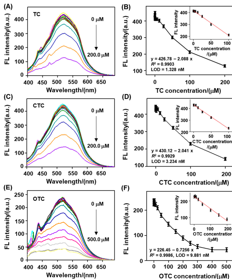
Figure 4. Fluorescence response of the biomass-based C-dots toward TCs in BR buffer. (A) Fluorescence emission spectra of the biomass-based C-dots (25.0 µg/mL) incubated with various concentrations of TC in the range of 0.0 to 200.0 µM. (B) C-dots fluorescence intensity plot at 520 nm versus TC concentration, as shown in Figure 4A. Inset: linearity of the C-dots fluorescence intensity at 520 nm versus CTC concentration in the range of 0.0–100.0 µM. Conditions: pH = 5.0; reaction time, 10.0 min; temperature, 20.0 °C. (C) Fluorescence emission spectra of the biomass-based C-dots (25.0 µg/mL) incubated with various concentrations of CTC in the range of 0.0 to 200.0 µM. (D) C-dots fluorescence intensity plot at 520 nm versus CTC concentration, as shown in Figure 4C. Inset: linearity of the C-dots fluorescence intensity at 520 nm versus CTC concentration in the range of 0.0–100.0 µM. Conditions: pH = 4.0; reaction time, 10.0 min; temperature, 50.0 °C. (E) Fluorescence emission spectra of the biomass-based C-dots (10.0 µg/mL) incubated with various concentrations of OTC in the range of 0.0 to 500.0 µM. (F) C-dot fluorescence intensity plot at 520 nm versus OTC concentration, as shown in Figure 4E. Inset: linearity of the C-dots fluorescence intensity at 520 nm versus OTC concentration in the range of 0.0–200.0 µM. Conditions: pH = 4.0; reaction time, 10.0 min; temperature, 20.0 °C.
