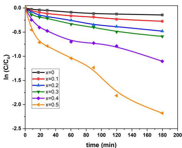
Figure 7. Variation of \ln C/C_0 vs time for (\text{Mn}_{0.5}\text{Zn}_{0.5})[\text{Cd}_x\text{Fe}_{2-x}]\text{O}_4 ( x = 0.1, 0.3 and 0.5 ) NSF s.
