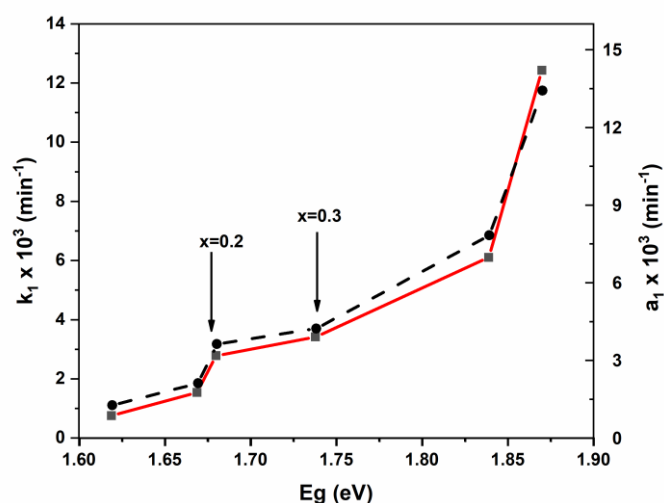
Figure 13. Variation of pseudo rate constant ( k_1 ) and modified pseudo-rate constant ( a_1 ) vs. bandgap energy.
