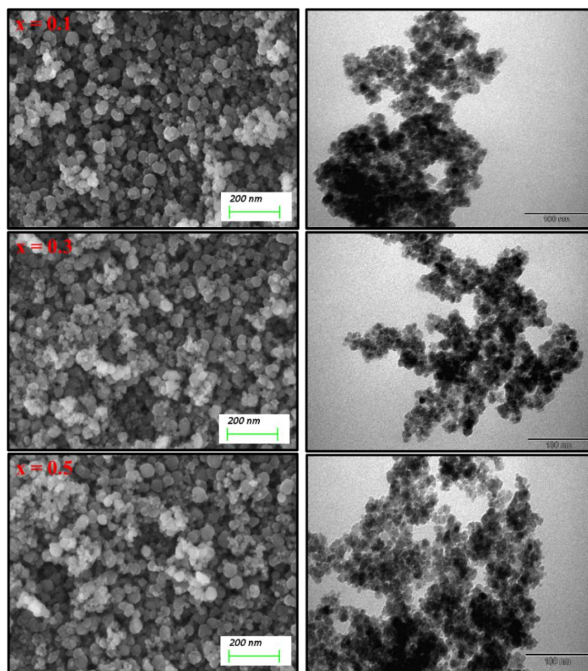
Figure 2. SEM and TEM images of (\text{Mn}_{0.5}\text{Zn}_{0.5})[\text{Cd}_x\text{Fe}_{2-x}]\text{O}_4 ( x = 0.1, 0.3 and 0.5 ) NSFs.
