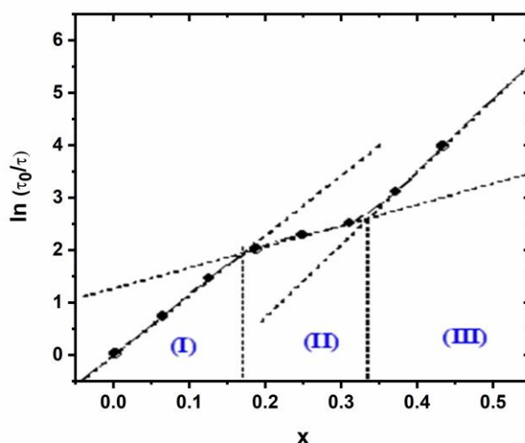
Figure 12. Variation of \ln(\tau/\tau_0) as a function of ( x ).
