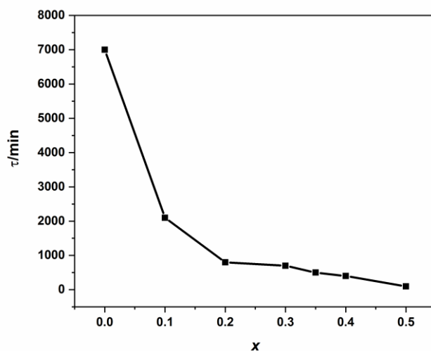
Figure 11. Variation of intra-diffusion time \tau vs. cadmium coordination in NSFs.
