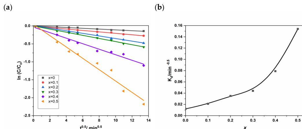
Figure 10. (a) \ln(C/C_0) for different as a function t^{1/2} and (b) K_d vs. cadmium coordination in NSF.
