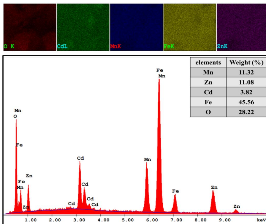
Figure 3. EDX and elemental mapping of (\text{Mn}_{0.5}\text{Zn}_{0.5})[\text{Cd}_x\text{Fe}_{2-x}]\text{O}_4 ( x = 0.2 ) NSFs.
