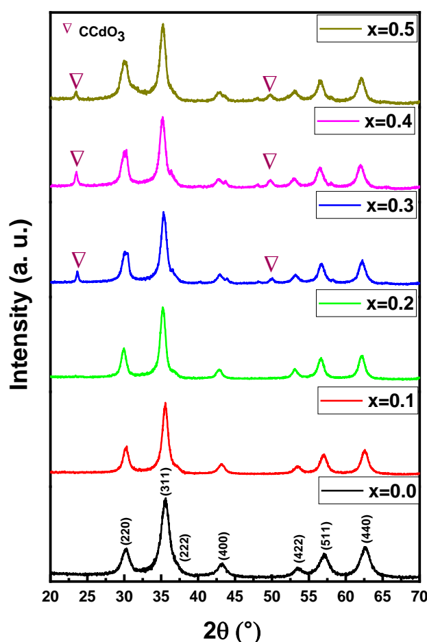
Figure 1. XRD powder patterns of (\text{Mn}_{0.5}\text{Zn}_{0.5})[\text{Cd}_x\text{Fe}_{2-x}]\text{O}_4 ( x \leq 0.05 ) NSFs.
