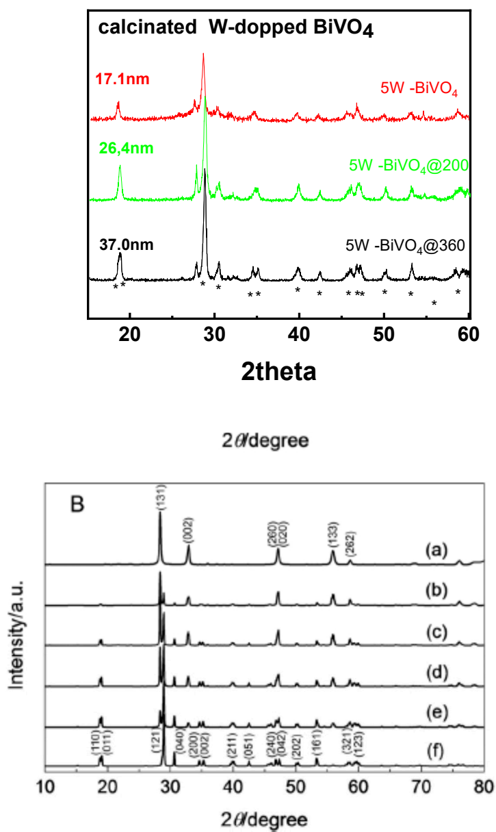
Figure S2. XRD pattern of calcined W-doped \text{BiVO}_4 .
