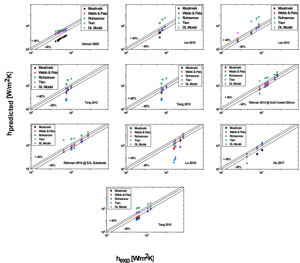
Figure 12. Predictions with correlations available in literature and DL Model.
