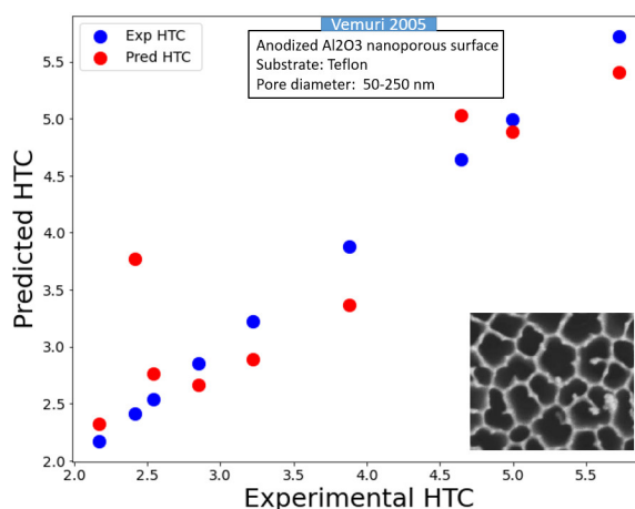
Figure 10. Assessment of various nanoporous coated surfaces available in the literature (note that HTC was taken in \text{kW/m}^2\cdot\text{K} ).
