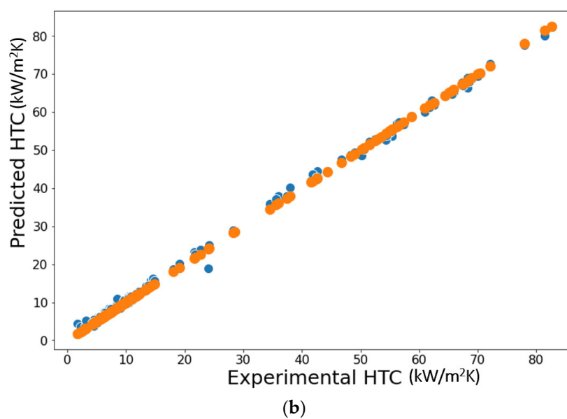
Figure 7. Predictions of the proposed model, (a) training and testing datasets and (b) testing dataset.
