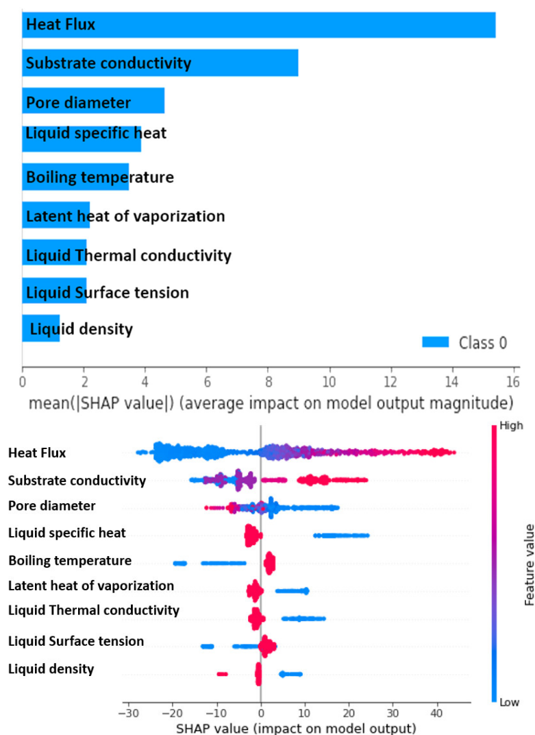
Figure 13. Sensitivity analysis.
