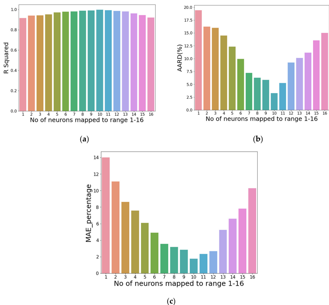
Figure 9. Variation in (a) R^2 , (b) AARD%, and (c) MAE% with the different number of dense neurons.
