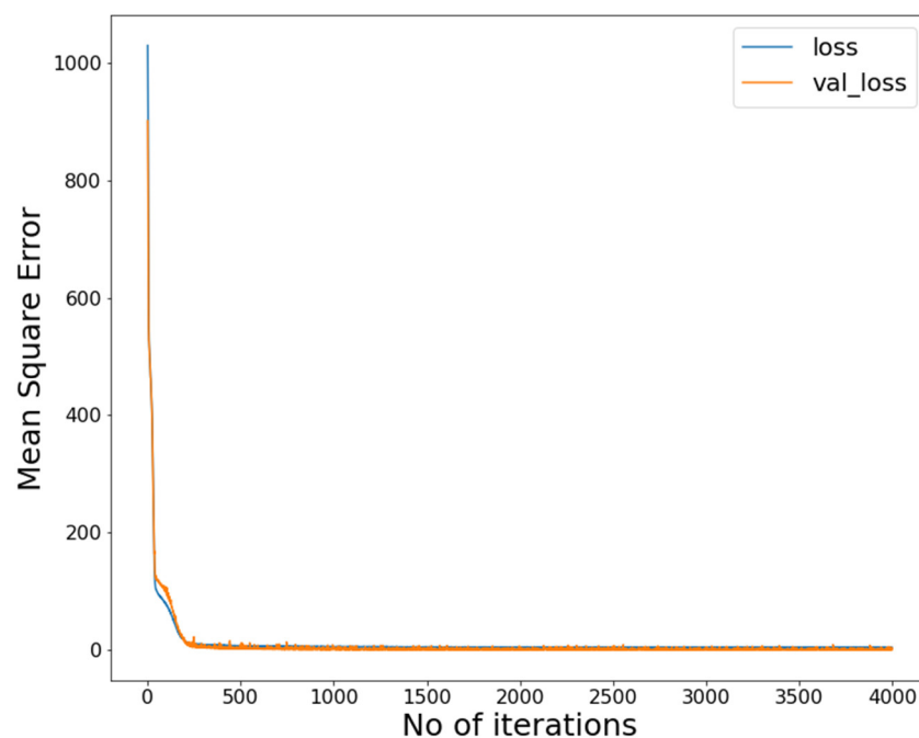
Figure 6. MSE trend.
