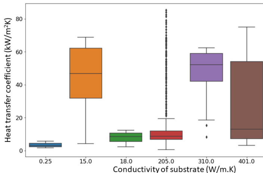
Figure 2. Heat transfer coefficient vs. thermal conductivity of substrate material.
