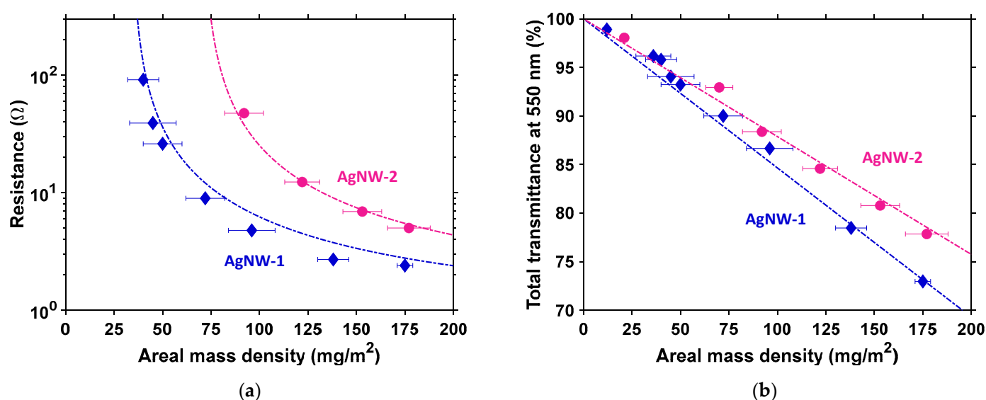
Figure 2. (a) Dependency of resistance, R , of the AgNW network versus amd ; (b) Dependency of the total transmittance, Tr , of the AgNW network versus amd . Symbols (blue diamond and pink circle) correspond to experimental data of AgNWs (AgNW-1 and AgNW-2, respectively), while dashed lines correspond to R and Tr fitting using Equation (2) and Equation (3), respectively. The substrate contribution was removed.
