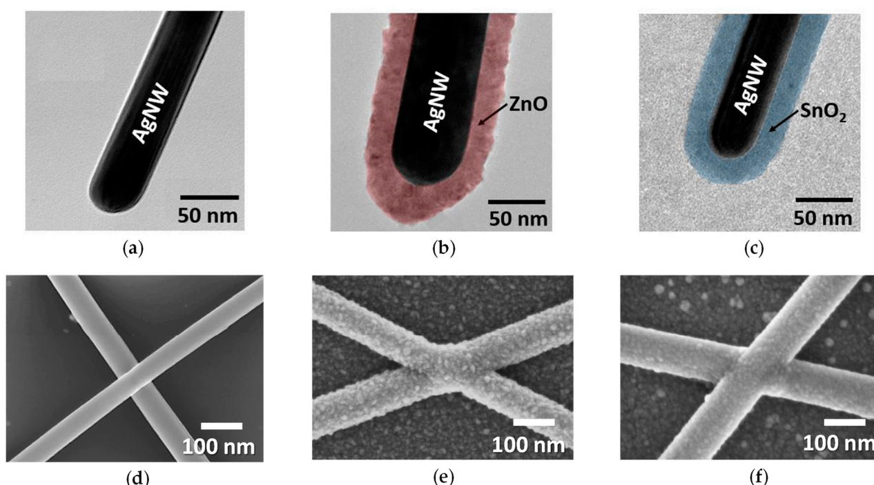
Figure 5. Coating AgNWs with thin oxide films by AP-SALD. TEM observations of (a) bare AgNW; (b) \text{ZnO}/\text{AgNW} and (c) \text{SnO}_2/\text{AgNW} nanocomposites. SEM observations of (d) bare AgNW; (e) \text{ZnO}/\text{AgNW} and (f) \text{SnO}_2/\text{AgNW} nanocomposites. The ZnO and \text{SnO}_2 coating thicknesses around the AgNWs were about 25 nm.
