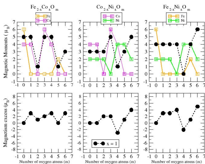
Figure 12. (upper panels) Total magnetic moments of A_{2-x}B_xO_m clusters ( A, B = Fe, Co, Ni ; x \leq 2 ; m = 1-6 ). Brown, pink and green curves correspond, respectively, to Fe_nO_m , Co_nO_m and Ni_nO_m oxides. Black curves correspond to nanoalloys with x = 1 . (lower panels) Magnetism excess of ABO_m nanoalloys ( A, B = Fe, Co, Ni ; m = 1-6 ).
