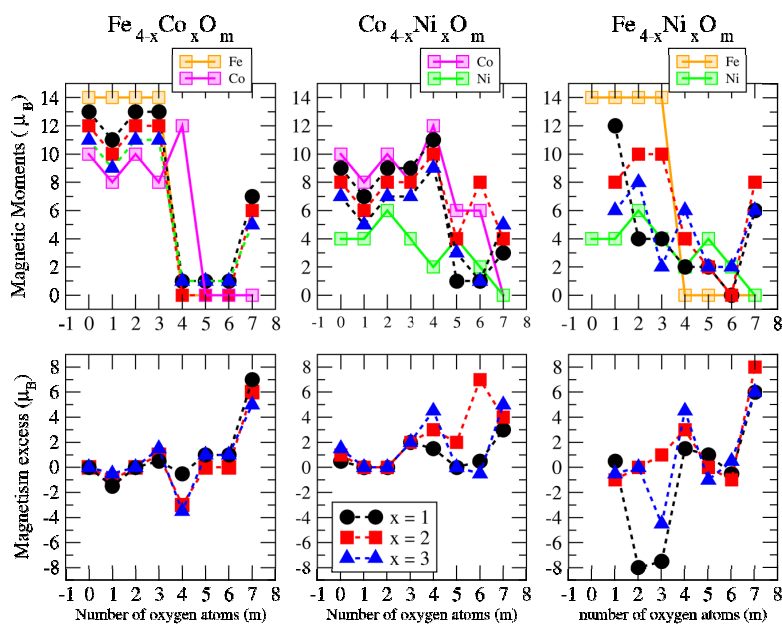
Figure 14. (upper panels) Total magnetic moments of A_{4-x}B_xO_m clusters ( A, B = \text{Fe, Co, Ni} ; 0 \leq x \leq 4 ; m = 1-7 ). Brown, pink and green curves correspond, respectively, to \text{Fe}_n\text{O}_m , \text{Co}_n\text{O}_m and \text{Ni}_n\text{O}_m oxides. Black, red and blue curves correspond to nanoalloys with x=1, 2, 3 , respectively. (lower panels) Magnetism excess of A_{4-x}B_xO_m clusters ( A, B = \text{Fe, Co, Ni} ; 1 \leq x \leq 3 ; m = 1-7 ).
