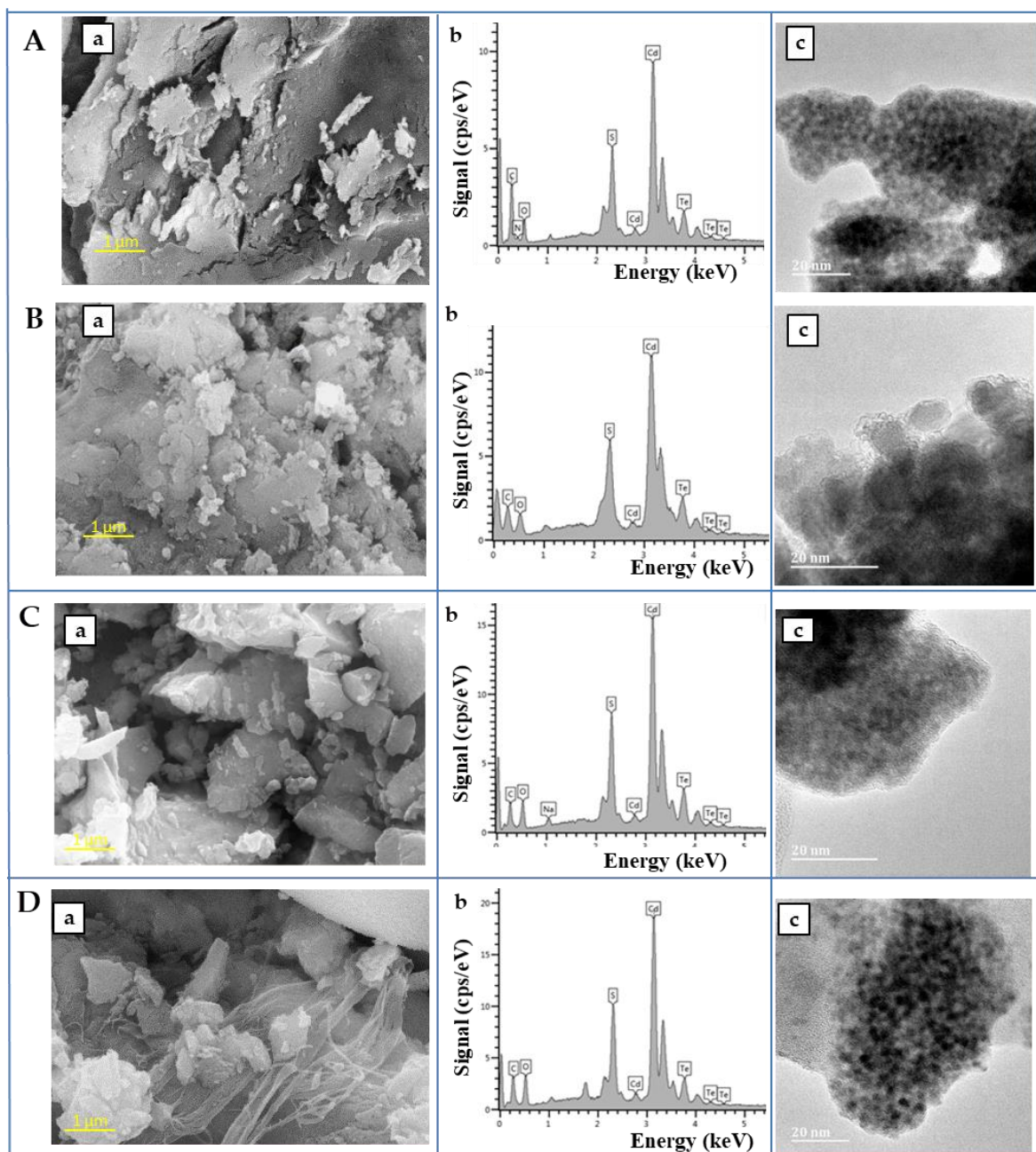
Figure S1. SEM (a), EDX elemental mapping (b) and HRTEM (c) of CdTe quantum dots (QDs). (A) Yellow, (B) green, (C) red and (D) orange CdTe QDs. Further experimental details are described in the Materials and Methods section.
