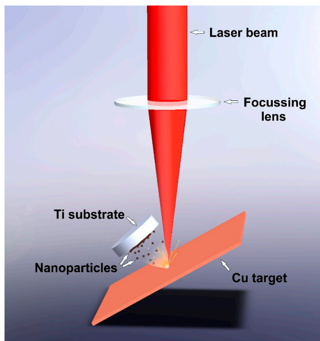
Figure 1. Laser ablation process.
