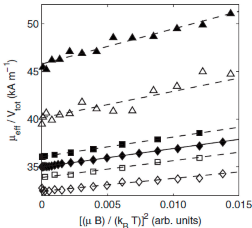
Figure 26. MMC effective magnetic moment dependence on the field induction square for several types of constituent nanoparticles. (Reprinted figure from [269]. Copyright 2009 by the American Physical Society.)
