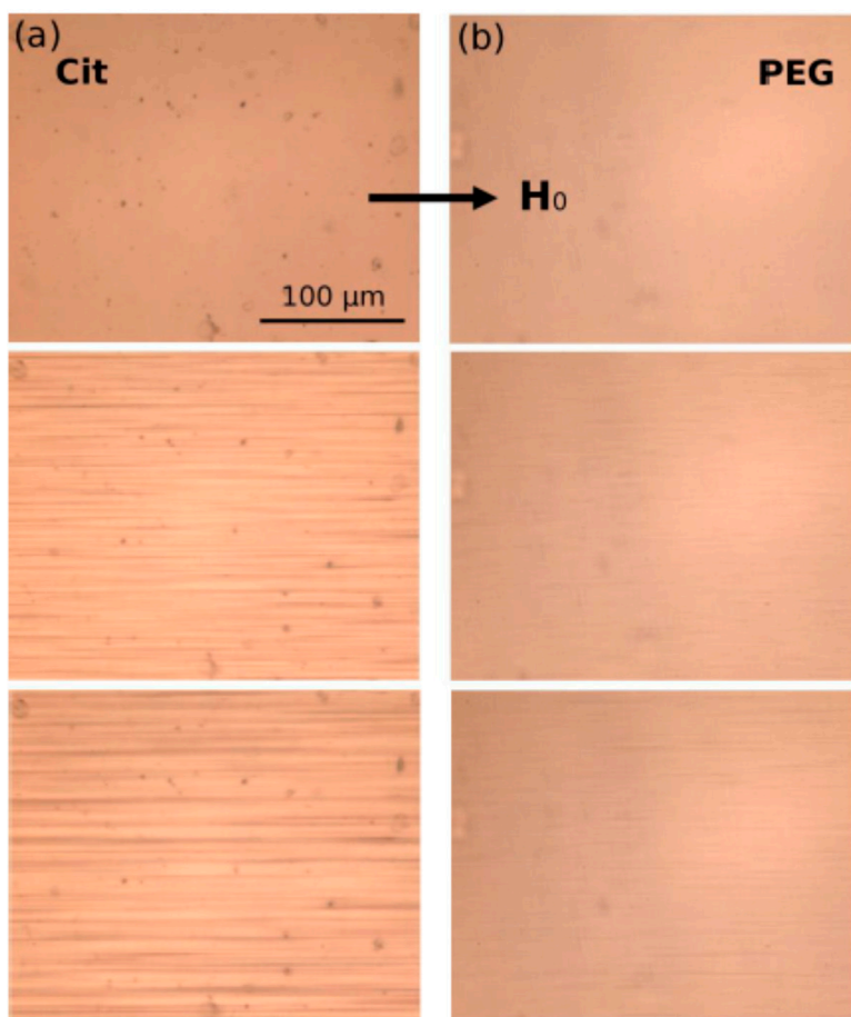
Figure 28. Optical microscopy images of aqueous suspensions of a) citrated, and b) PEGylated MNCs in an external uniform DC magnetic field of intensity 13.5 kA/m. Each row corresponds to the elapsed time from the moment of the magnetic field application t = 0 (upper row), 5 and 10 min. (Reprinted from [274] under Open Access license).
