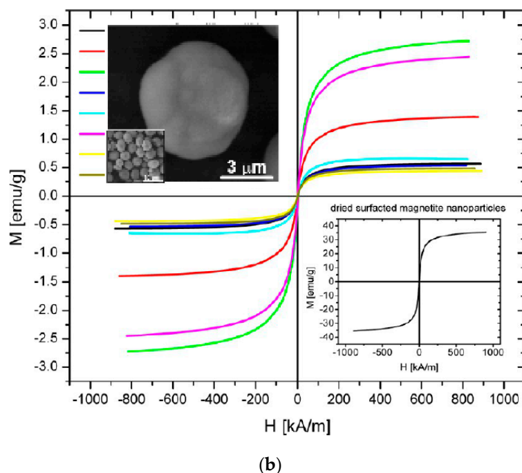
Figure 24. (a) Magnetic multi-core particle (reprinted from [77], Copyright 2015, with permission from Elsevier), and (b) Magnetization curves of the dried composite microparticles. Inset shows the magnetization of the dried surface coated magnetite nanoparticles. (Reprinted with permission from [167]. Copyright 2013 American Chemical Society.).
