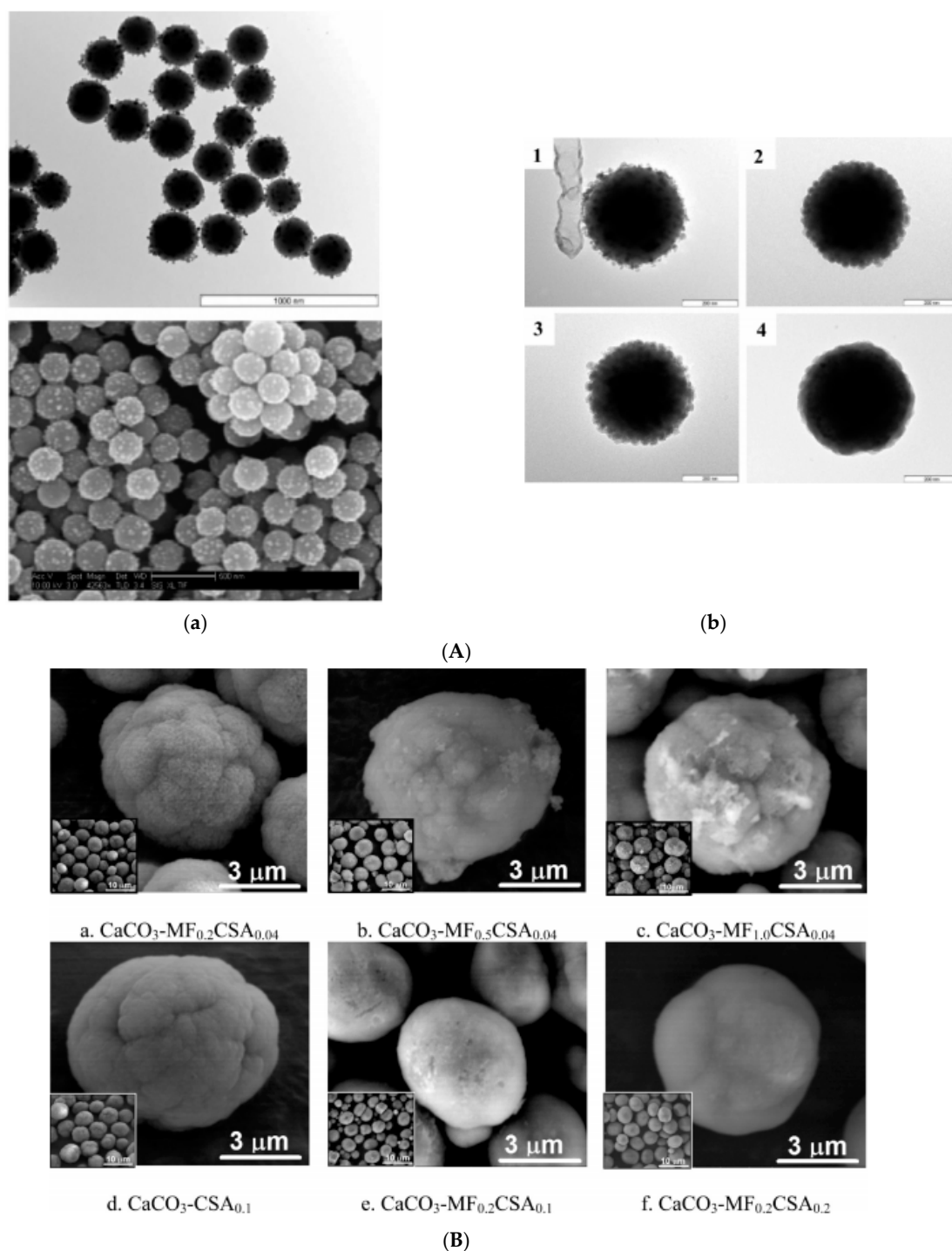
Figure 7. (A) (a) TEM (top) and corresponding SEM picture (bottom) of silica-cobalt ferrite nanocomposite particles (b) Silica growth onto composite particles monitored by TEM, which shows the gradually increasing silica layer thickness from no silica present in picture 1 to a fully grown silica layer in picture 4. (Reprinted with permission from [52] Copyright 2005 American Chemical Society). (B) Magneto-responsive chondroitin sulfate-functionalized CaCO 3 microparticles. The influence of CSA and magnetic fluid (MF) content on the CaCO 3 -MF-CSA composite size, shape, and morphology, as evidenced by SEM (reprinted with permission from [167]. Copyright 2013 American Chemical Society).
