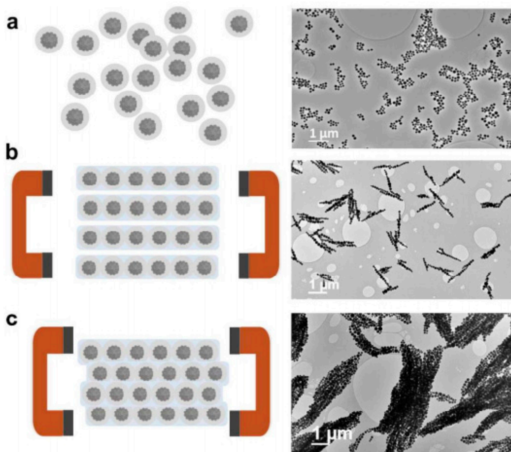
Figure 9. Schematic representation of the fabrication process (left-hand image) and the corresponding transmission electron microscopy images (right-hand image) of (a) silica-coated superparamagnetic nanoparticle clusters, (b) nanochains, and (c) nanobundles (reprinted with permission from [177]. Copyright 2015 American Chemical Society).
