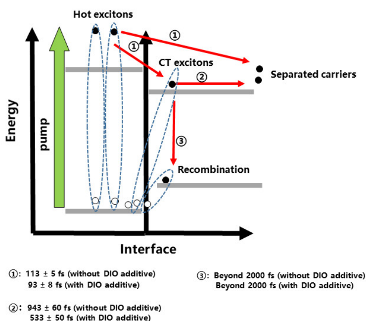
Figure 6. A schematic of ultrafast interfacial excitons dynamics in the P51:PC 71 BM blend after photoexcitation. ①: Charge Transfer (CT) excitons and free charge generation from hot excitons; ②: dissociation of CT excitons into free charge carriers; ③: recombination decay of photocarriers.
