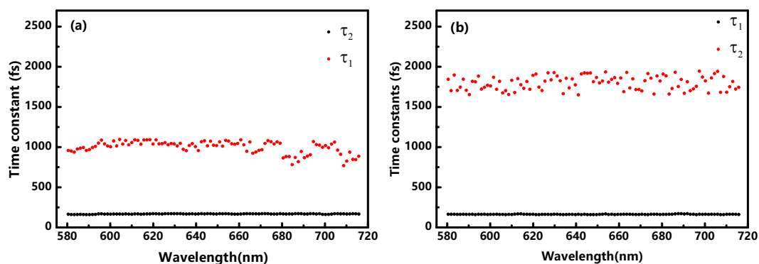
Figure 3. Time constants obtained by a calculation using a two-exponential function for (a) P51 without DIO additives; (b) P51 with DIO additives.
