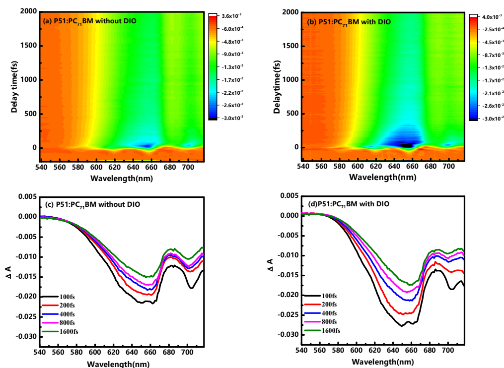
Figure 4. Two-dimensional plot of transient difference absorption \Delta A(\lambda, t) and \Delta A(\lambda) spectra at various time delays for (a,c) P51:PC 71 BM without DIO additives and (b,d) P51:PC 71 BM with DIO additives.
