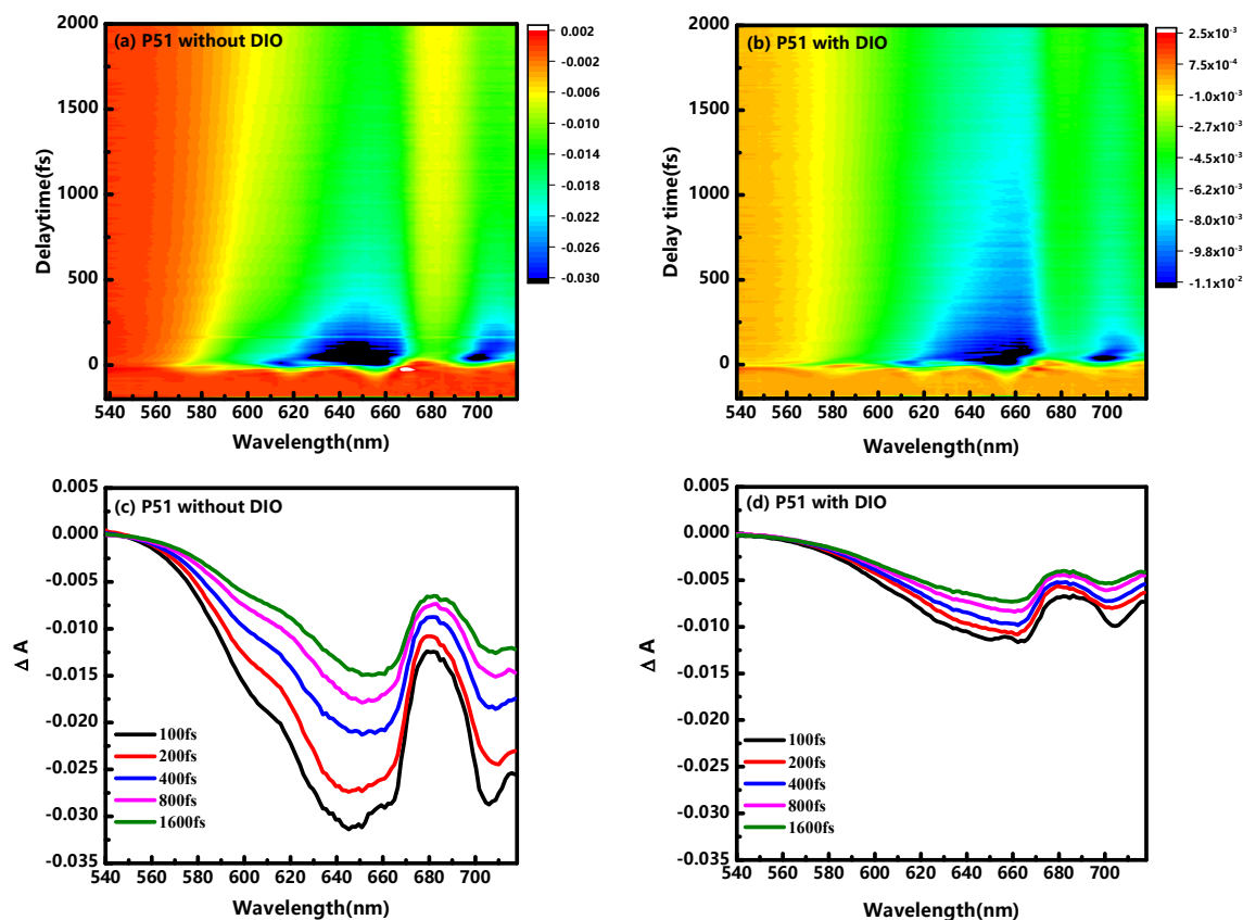
Figure 2. Two-dimensional plot of transient difference absorption \Delta A(\lambda, t) and \Delta A(\lambda) spectra at various time delays for (a,c) pristine P51 without DIO additives and (b,d) pristine P51 with DIO additives.
