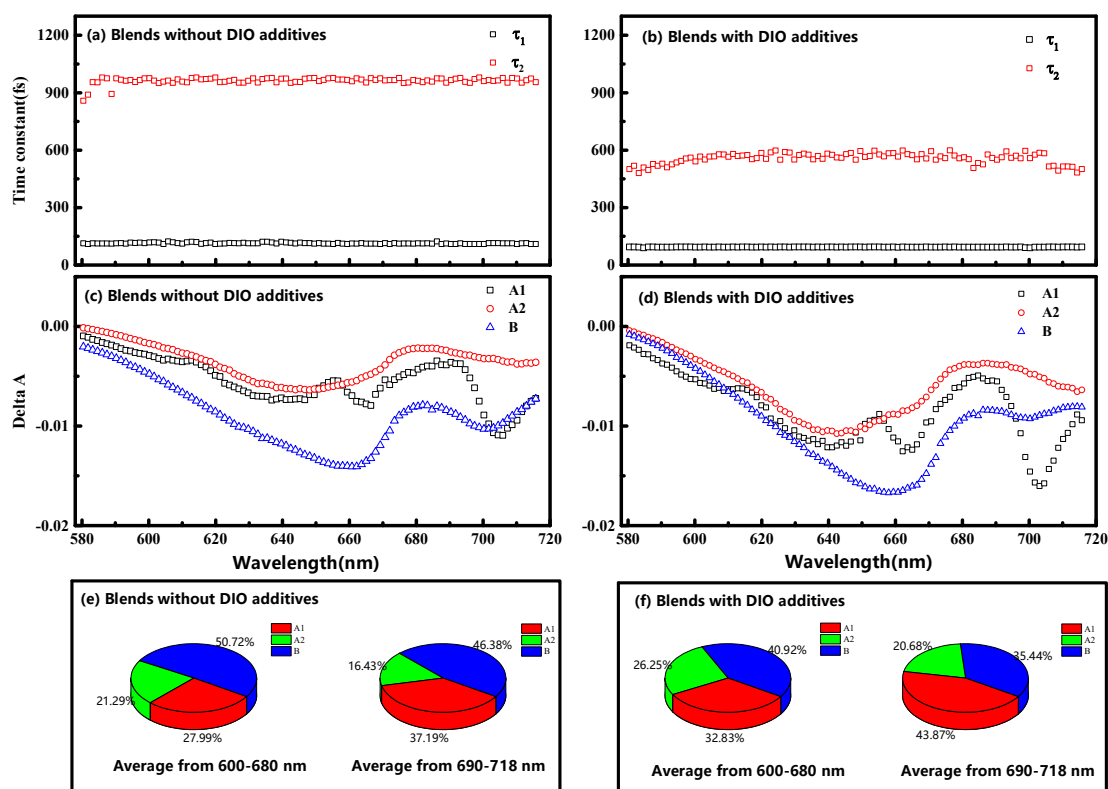
Figure 5. Fitting results with the two-exponential function for the time traces: (a) P51:PC 71 BM blends without DIO additives; (b) P51:PC 71 BM blends with DIO additives; (c) decomposed A1, A2 and B in (c) blends without DIO additives (d) blends with DIO additives. (e) Percent of A1, A2 and B in blends without DIO additives; (f) percent of A1, A2 and B in blends with DIO additives.
