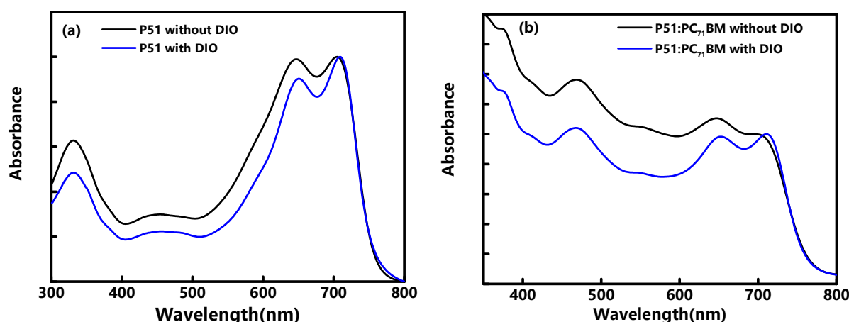
Figure 1. (a) Steady-state absorption spectra of the pristine P51 with/without 1,8-diiodooctane (DIO) additive; (b) steady-state absorption spectra of P51:PC 71 BM blend with/without DIO additive.
