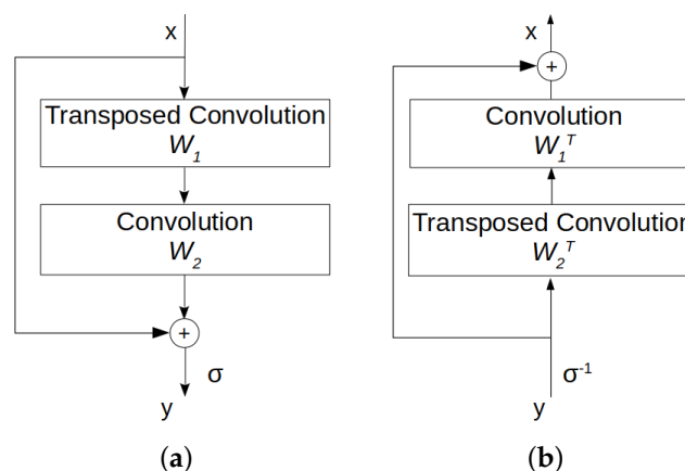
Figure 3. (a) Residual block. (b) Inverted residual block.
