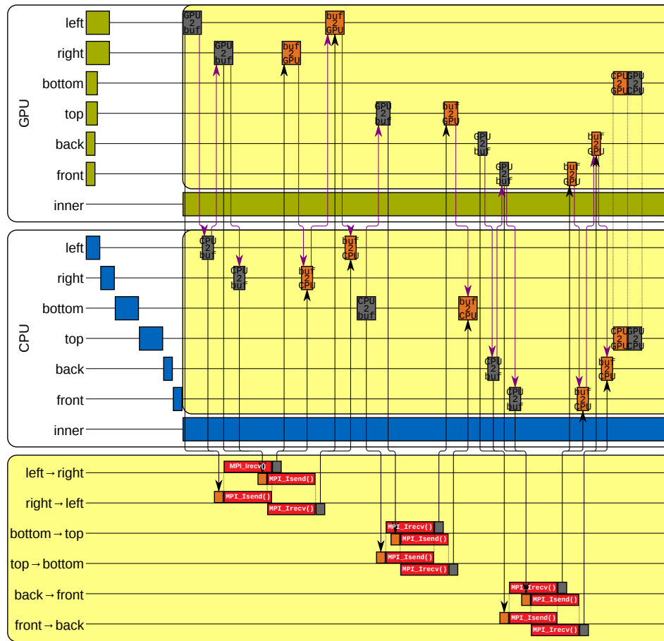
Figure 7. Timeline of one MPI process during an \alpha - or \beta -step [19]. Operations are grouped in GPU (top), CPU (middle), and MPI (bottom) activities. Within each computing device's group, operations affecting the six faces and the inner cells are illustrated. Communication and copy actions are highlighted by yellow background, computations by white background. Green and blue bars indicate computations on the GPU and CPU. Red bars symbolize MPI communication distinguished between sending (MPI_Isend()) and receiving (MPI_Irecv()). Communication directions are denoted by "from ...neighbor \rightarrow ...boundary layer". Grey and orange bars represent memory transfers to and from the communication buffers stored on the host, respectively. Bars marked with "GPU2buf" perform a copy operation from the GPU to the communication buffers and those with "CPU2buf" from the CPU to the communication buffers. The copy operations from the communication buffers to the computing devices are marked with "buf2GPU" and "buf2CPU". Copy operations along the interface between CPU- and GPU-part of the subdomain are called "CPU2GPU" and "GPU2CPU". Black arrows indicate data dependencies, purple arrows illustrate dependencies due to shared resources.
