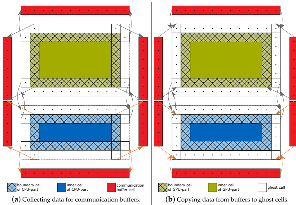
Figure 5. \alpha -step collection (a) and distribution (b) of data. The behavior of one MPI process with four communication partners is illustrated in 2D. GPU- and CPU-part of the subdomain are colored in green and blue. Boundary cells are hatched and colored in light-green and light-blue, ghost cells are colored in white. Memory for the communication buffers is colored in red. Gray arrows indicate copy direction between and location of host and device. Analogously, orange arrows express in-host memory copy operations. Lattice cells affected by read/write operations are marked with a dot.
