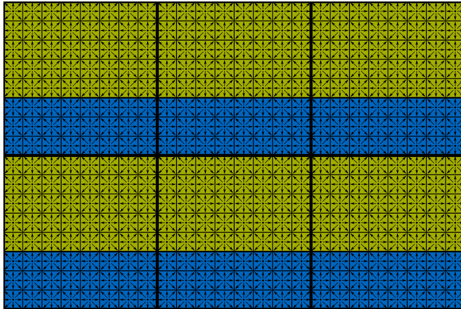
Figure 4. Decomposition of a 2D domain consisting of 24 \times 16 lattice cells in 3 \times 2 subdomains [19]. Each 8 \times 8 subdomain is subdivided in a 8 \times 5 upper part assigned to a GPU (green) and a 8 \times 3 lower part assigned to a CPU (blue).
