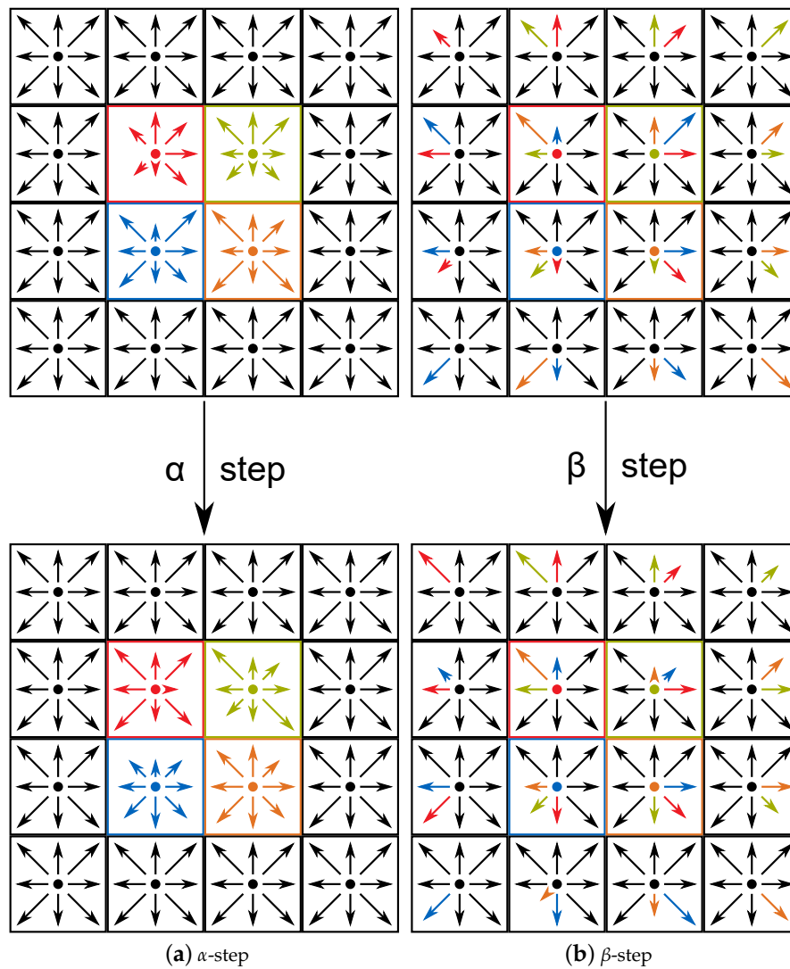
Figure 3. Probability densities of four processed cells (colored in red, green, blue, and orange) affected by memory accesses using the A-A memory layout pattern [19]. Different lengths of same-color arrows in the same direction represent an update of the probability densities due to a collision step. (a) Illustrates the \alpha -step consisting of one collision step, (b) depicts the \beta -step consisting of two propagation steps and one collision step.
