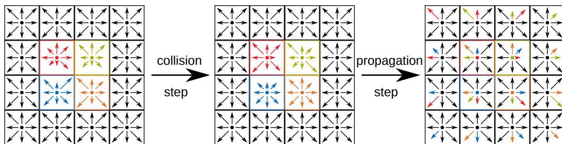
Figure 2. Probability densities of four processed cells (colored in red, green, blue, and orange) affected by collision and propagation steps [19]. Different lengths of same-color arrows in the same direction represent an update of the probability densities due to a collision step.
