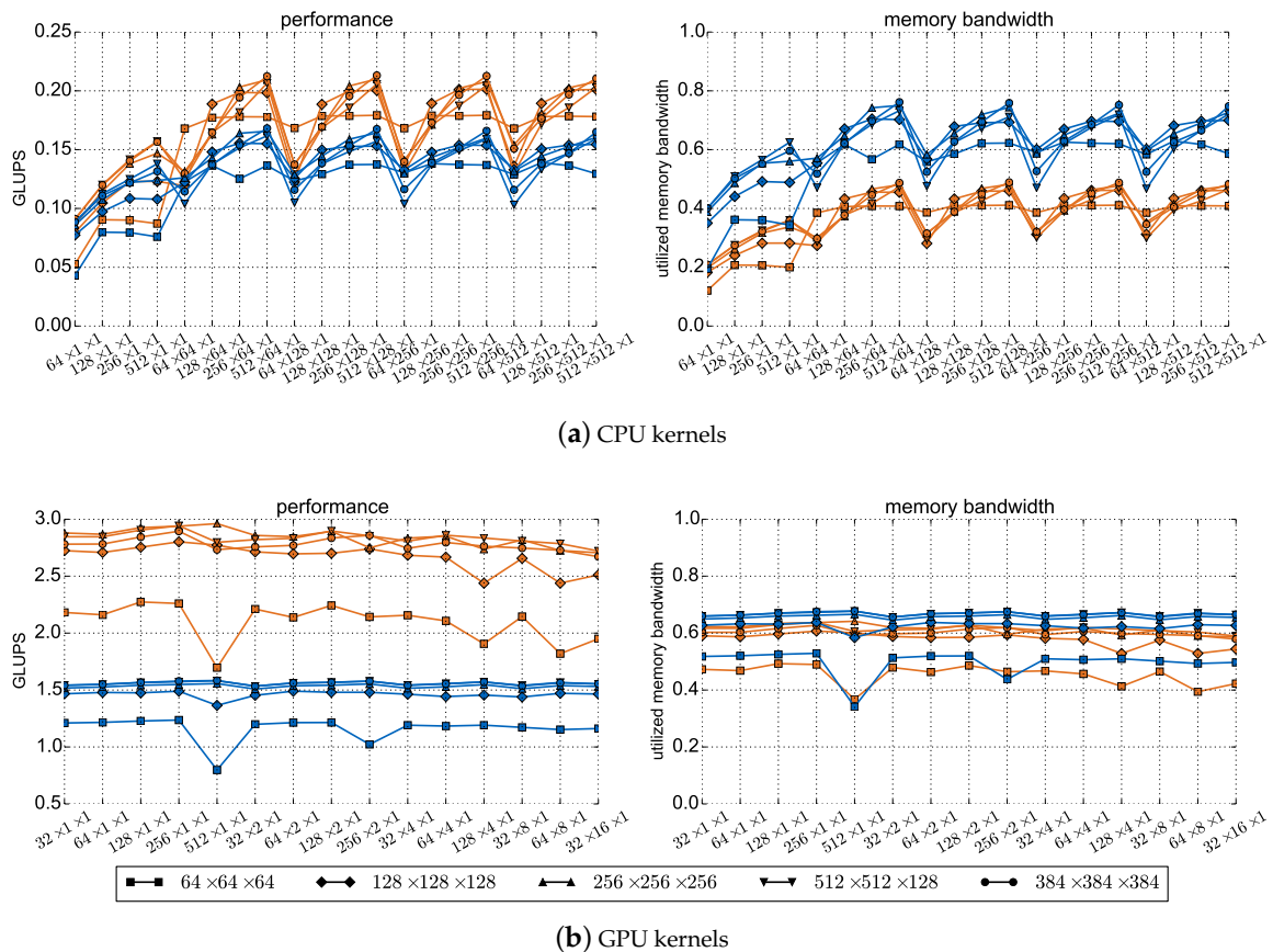
Figure 8. Performance in GLUPS (left) and share of utilized memory bandwidth in peak memory bandwidth (right). (a) Shows results for the CPU kernels, (b) for the GPU kernels. Values for the CPU depend on the block size used to increase cache efficiency and for the GPU on the parallel setup, each assigned to the abscissas. Different lines depict different problem sizes. Single precision (float) performance is colored in orange, double precision (double) performance in blue.
