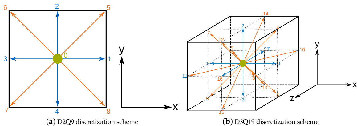
Figure 1. Discretization schemes for the LBM using q = 9 probability densities in 2D (a) and q = 19 probability densities in 3D (b), respectively [19]. Blue arrows represent probability densities with lattice speed c_i = 1 , red arrows with lattice speed c_i = \sqrt{2} , and green dots with lattice speed c_i = 0 . The orientation of the corresponding coordinate systems is indicated in the right parts of the subfigures.
