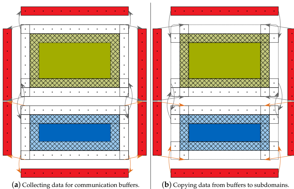
Figure 6. \beta -step collection (a) and distribution (b) of data. The behavior of one MPI process with four communication partners is illustrated in 2D. For color coding and meaning of data transfer arrows, see Figure 5. Lattice cells affected by read/write operations are marked with a dot.
