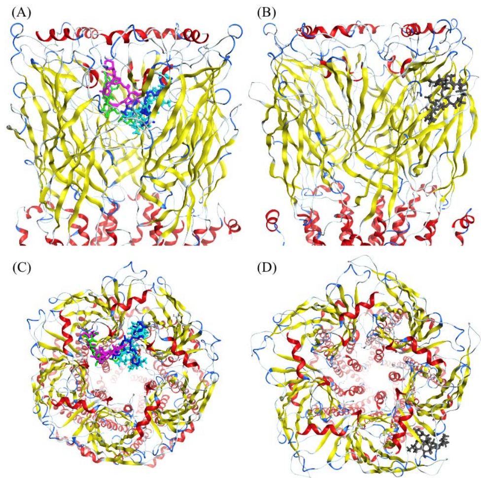
Figure 4. Binding poses of ivermectin (dark blue), doramectin (purple), okadaic acid (green), concanamycin A (cyan) on \alpha 7 nAChr (A) side and (C) top view. Binding pose of moxidectin (dark gray) on (B) side and (D) top view.
