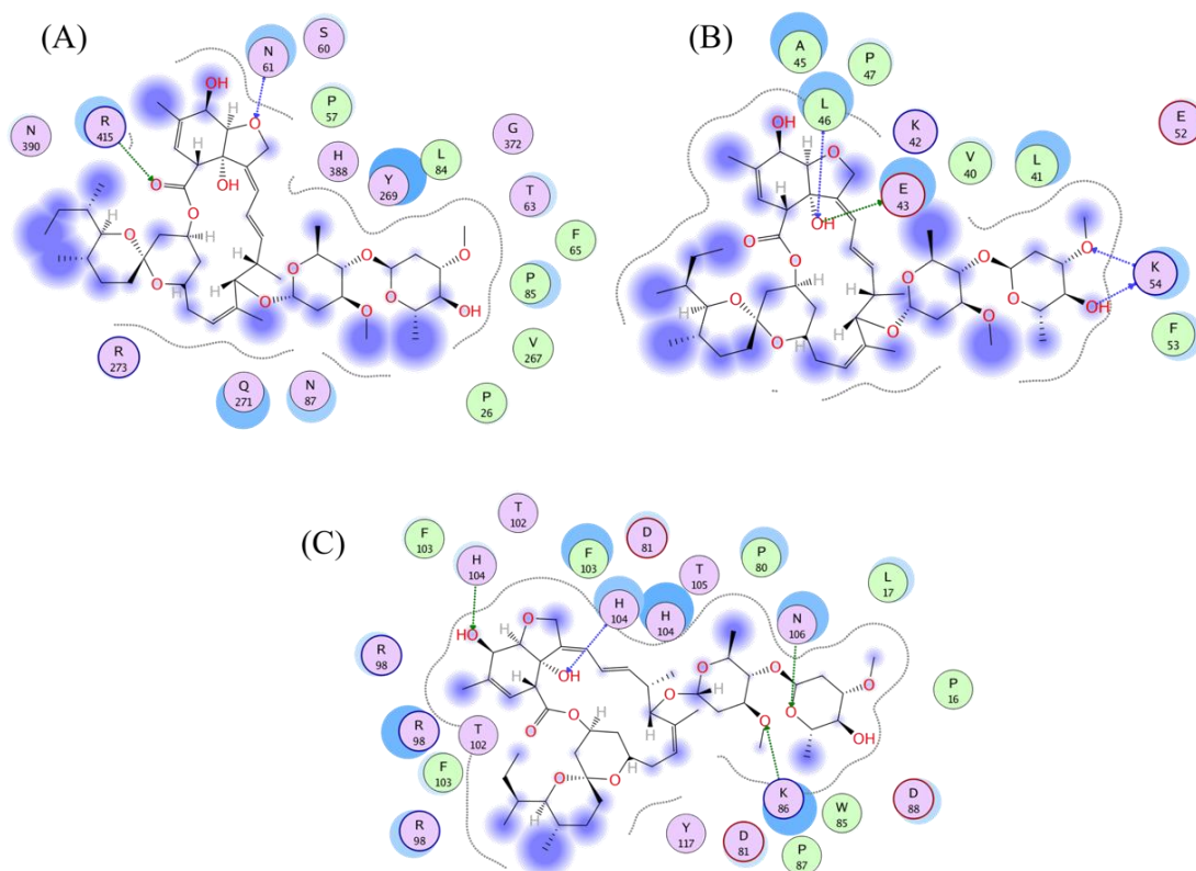
Figure 5. Ligand interaction plots of ivermectin for (A) spike, (B) CD147 and (C) \alpha 7\text{nAChr} inhibition.
