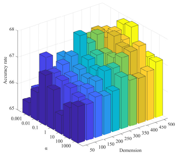
\alpha on ORL
