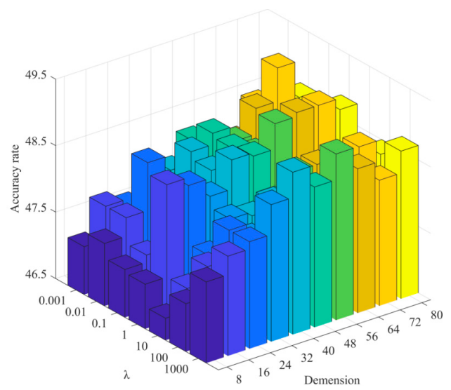
\lambda on Libras Movement
