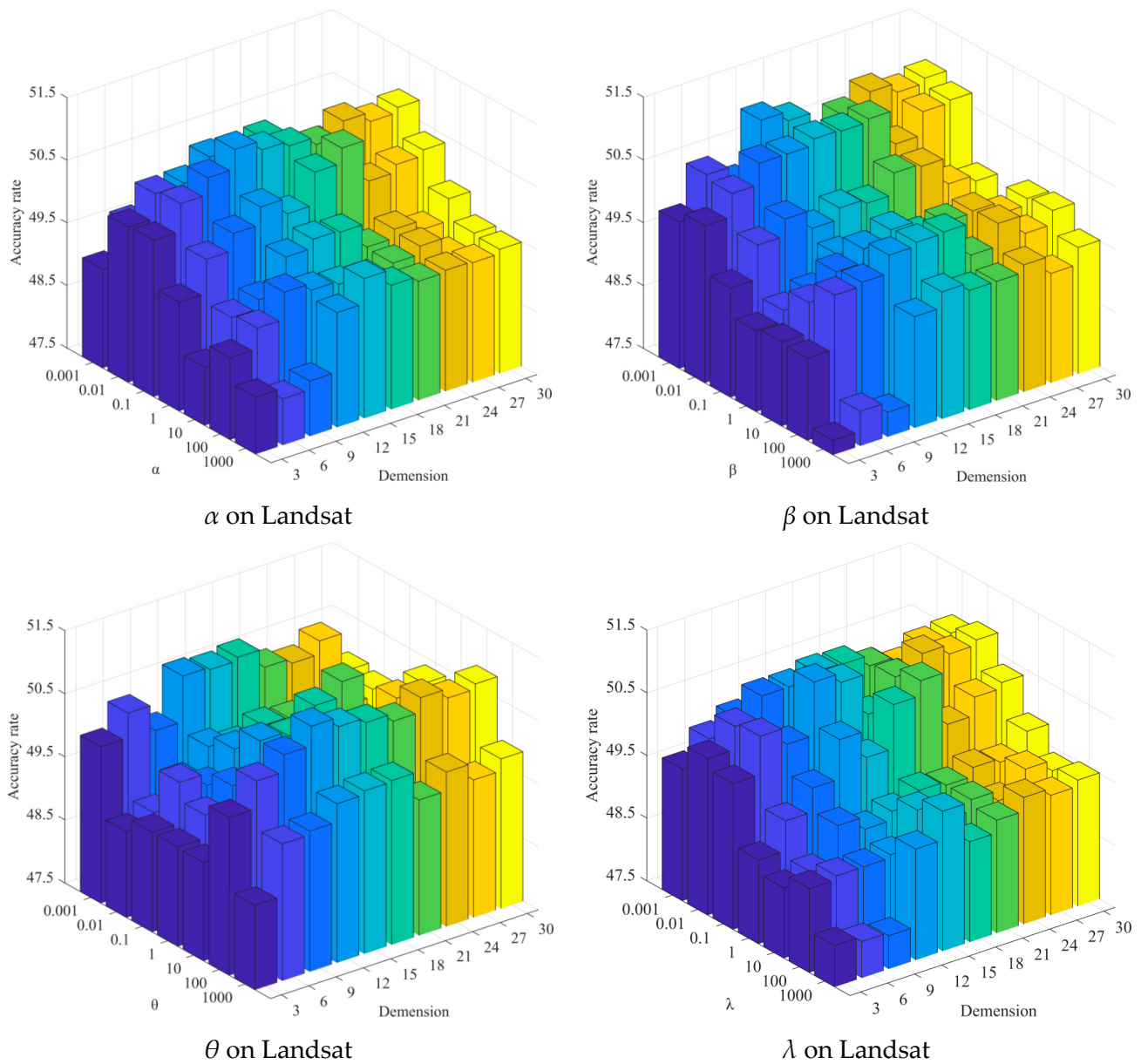
Figure 7. Clustering results of SFS-AGGL under different parameter values and different feature dimensions, where different colors represent different feature dimensions.
