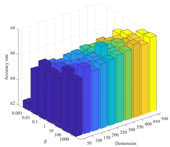
\beta on ORL
