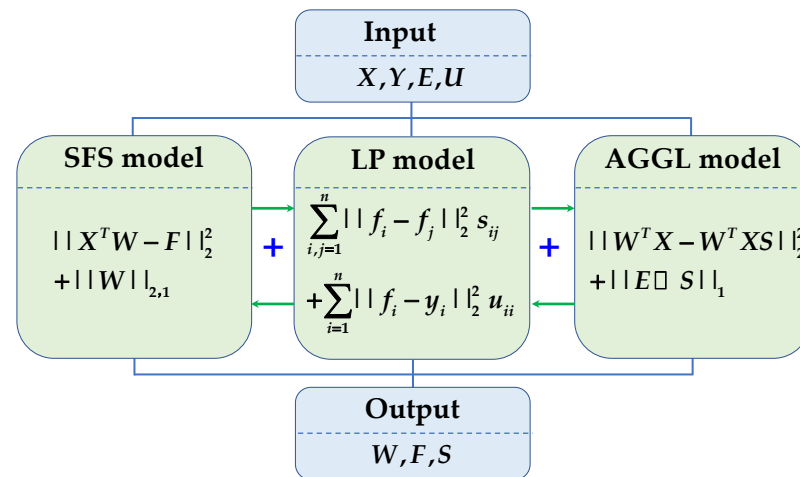
Figure 1. The illustration of the SFS-AGGL framework.
