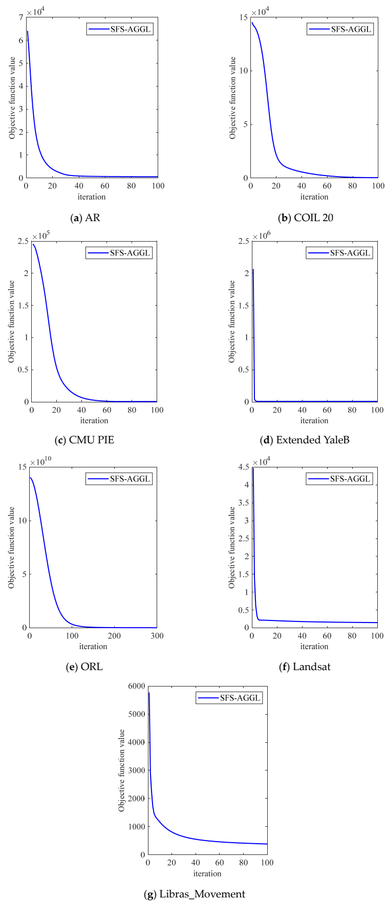
Figure 9. Convergence curves of SFS-AGGL on different datasets.
