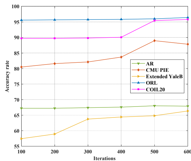
Figure 4. Classification accuracy of SFS-AGGL under different iterations.
