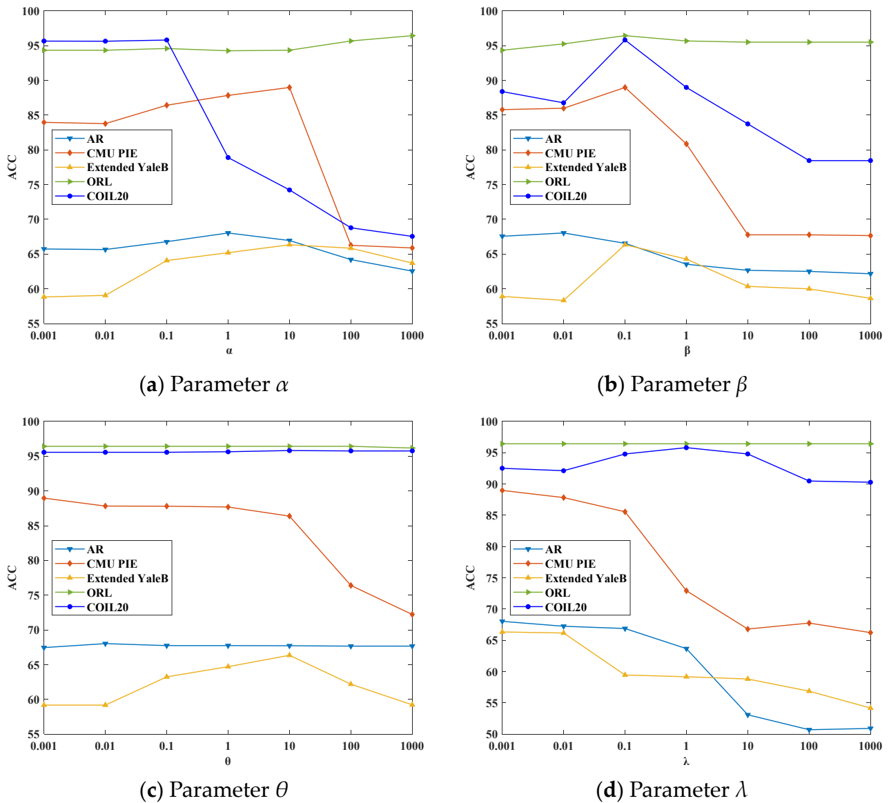
Figure 6. Classification results of SFS-AGGL under different parameter values.
