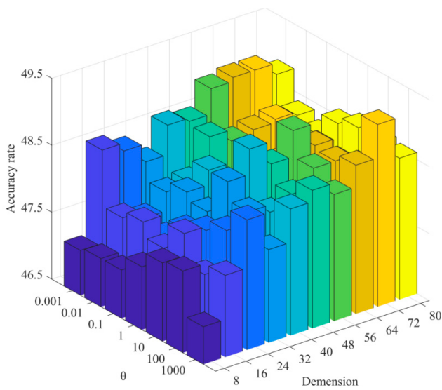
\theta on Libras Movement
