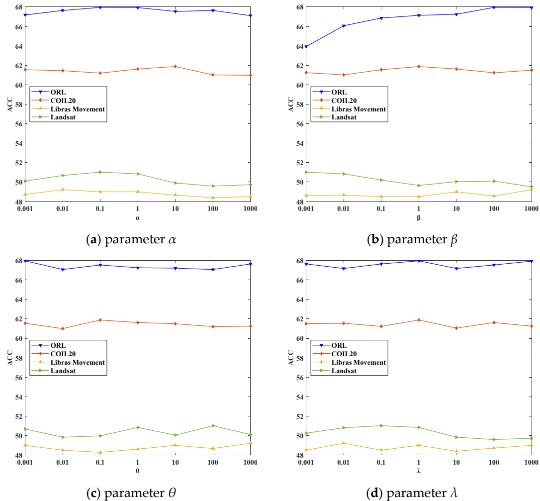
Figure 8. Clustering results of SFS-AGGL under different parameter values.
