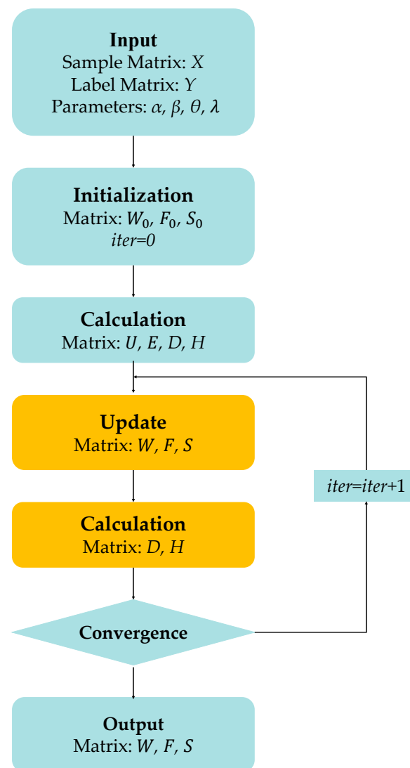
Figure 2. Flow chart of SFS-AGGL algorithm.
