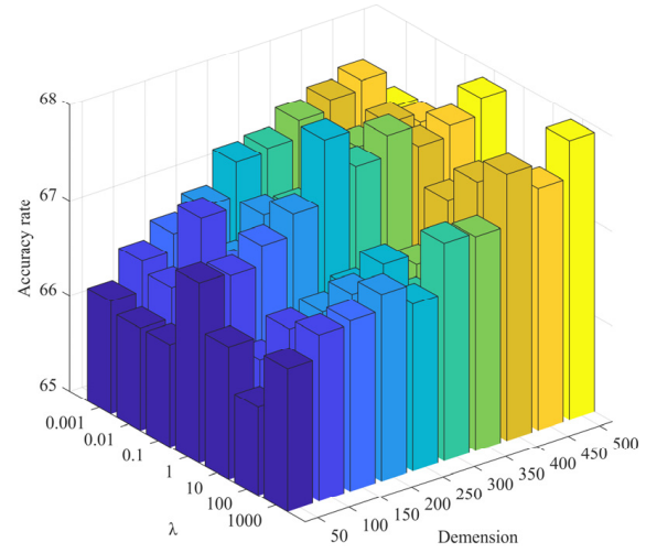
\lambda on ORL
