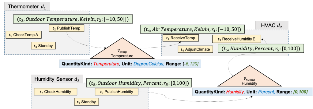
Figure 9. Service Design S_{HVAC} for an HVAC system of a smart farm.
