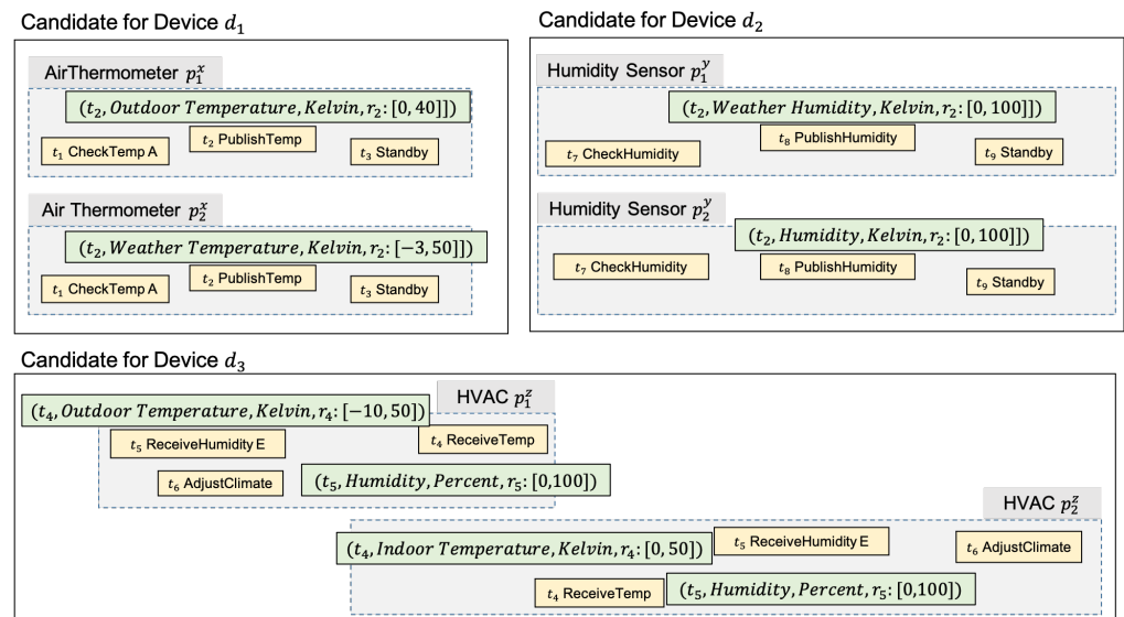
Figure 10. Example group of physical devices for S_{HVAC} .
