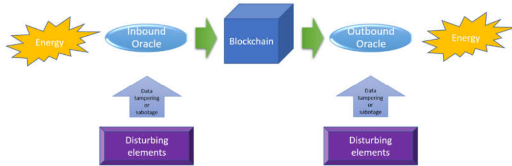
Figure 6. Example of the “dual” oracle problem.
