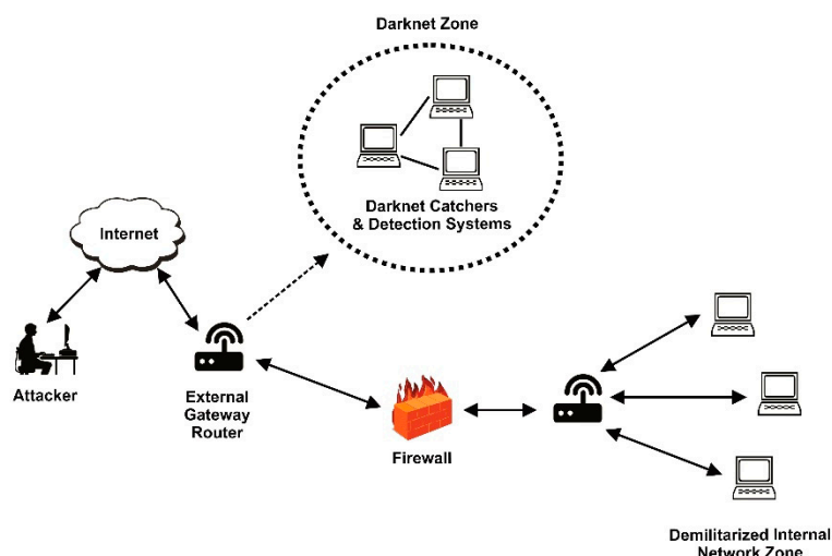
Figure 6. A basic deployment of a Darknet.
