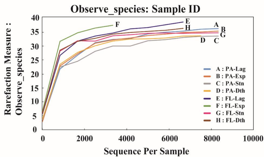
Figure S1. OTU counts (A) and rarefaction(B) of each growth phase of Tetraselmis suecica .
