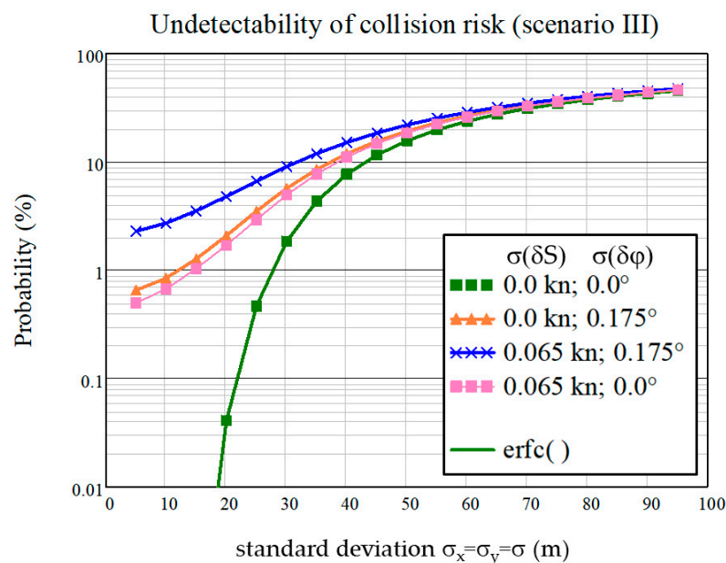
Figure 14. Impact of position, COG and SOG inaccuracies on the detectability of existing collision risks dependent on the standard deviation \sigma of position errors ( L = 100 m, provided for a forecast time \delta t = 18 min, equally distributed SOG values between 0 and 25 kn and equally distributed COG values between 0^\circ and 360^\circ ).
