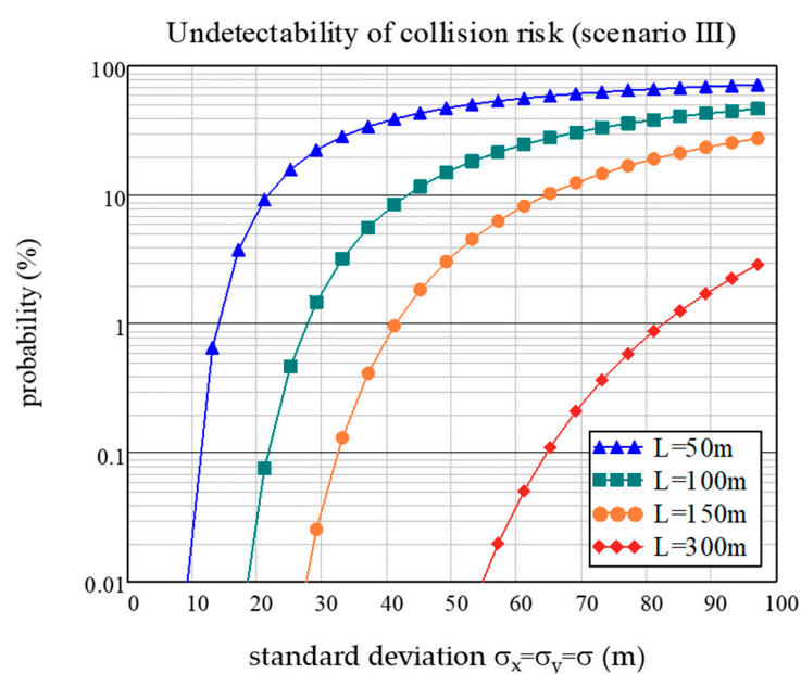
Figure 8. Undetectability of existing collision risks for exemplary diameters L of ship domains dependent on the assumed standard deviation of position error.
