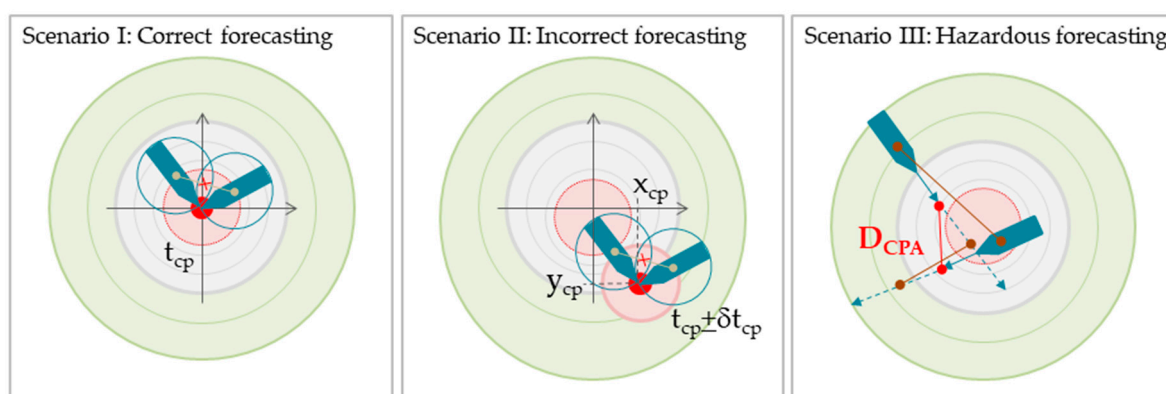
Figure 6. Impact of position, navigation and timing (PNT) data accuracy on the assessment of collision risk (collision area is marked with a red circle in case A and B; x_{cp} and y_{cp} —coordinates of collision point; D_{CPA} —distance between both ships at the closest point of approach (CPA)).
