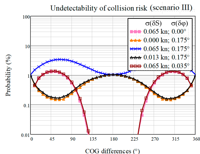
Figure 13. Impact of COG and SOG inaccuracies on the probability of undetected collisions risks dependent, on occurred COG differences \varphi_A - \varphi_B between both ships ( L = 100 m, provided for a forecast time \delta t = 18 min, equally distributed SOG values between 0 and 25 kn, and selected standard deviations \sigma(\delta \varphi) and \sigma(\delta S) ).
