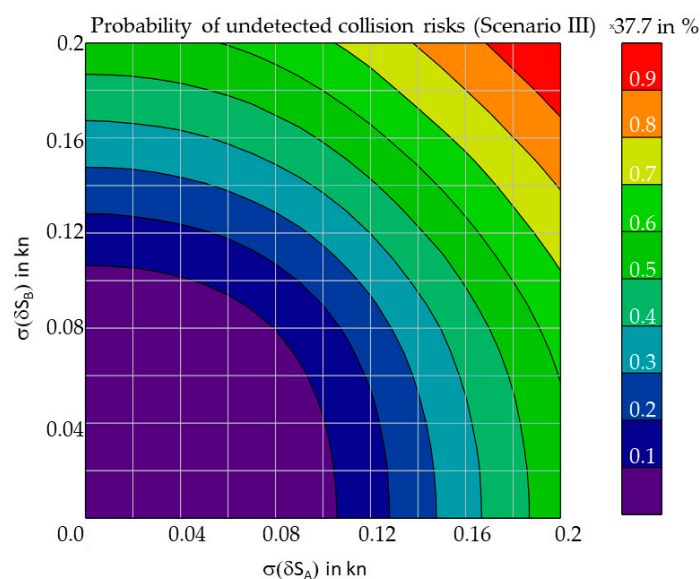
Figure 10. Probability of undetected collisions risks (colour-represented value range between 0 and 37.7%) dependent on the standard deviation of SOG inaccuracies with values between 0 and 0.2 kn ( \varphi_A - \varphi_B = +\pi/4 ; L = 100 m; \delta t = 18 min).
