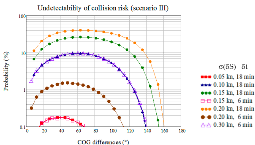
Figure 9. Impact of speed-over-ground (SOG) inaccuracies on the detectability of existing collision risks dependent on the COG differences \varphi_A - \varphi_B between both ships ( L = 100 m, provided for selected forecast times \delta t and standard deviations \sigma(\delta S_A) = \sigma(\delta S_B) = \sigma(\delta S) of SOG inaccuracies).
