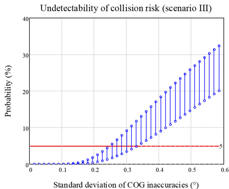
Figure 12. Range of probabilities of undetected collisions risks dependent on the standard deviation of COG inaccuracies ( L = 100 m, provided for a forecast time \delta t = 6 min and equally distributed SOG values between 0 and 25 kn).
