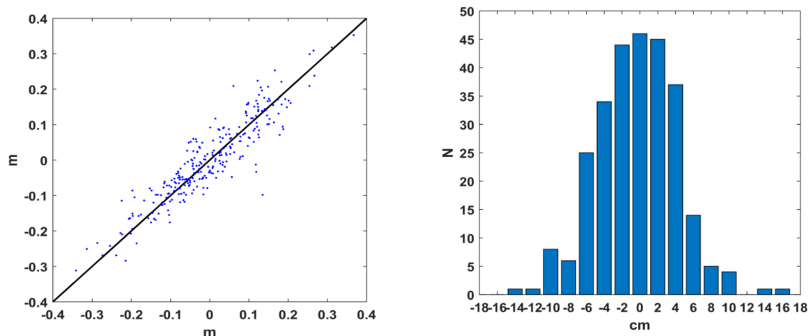
Figure 8. Plot of altimeter versus tidal gauge data ( left ) and distribution of their differences in classes of 2 cm each ( right ).
