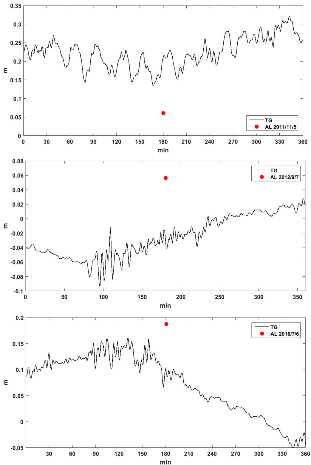
Figure 9. Time series of sea level data from the tidal gauge (black line) 3 h before and after the passage of the altimeter and the TWLE values detected by the altimeter (red dot).
