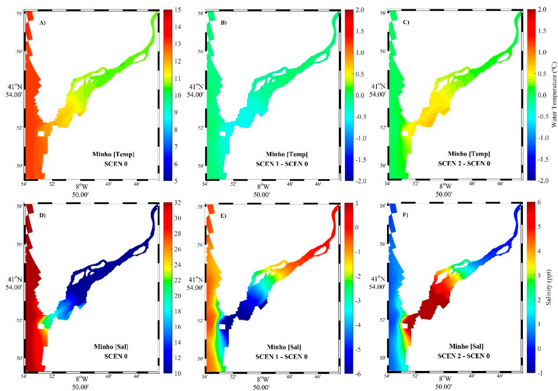
Supplementary Figure 3 (Fig. S3) - Mean water temperature (A, B, C), salinity (D, E, F) for Minho estuary in the winter season for the different scenarios.
