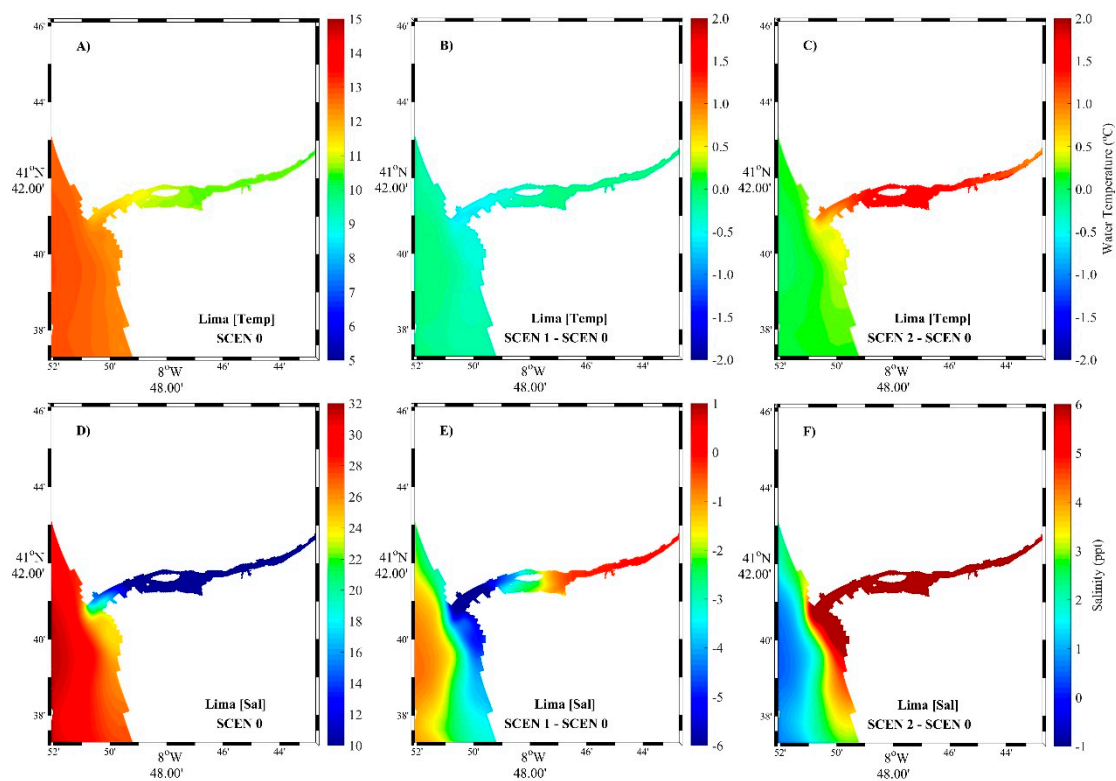
Supplementary Figure 4 (Fig. S4) - Mean water temperature (A, B, C), salinity (D, E, F) for Lima estuary in the winter season for the different scenarios.
