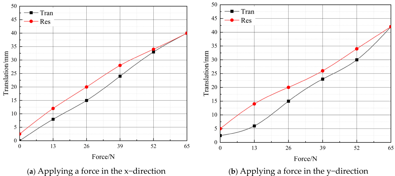
Figure 8. Restoring force curve.
