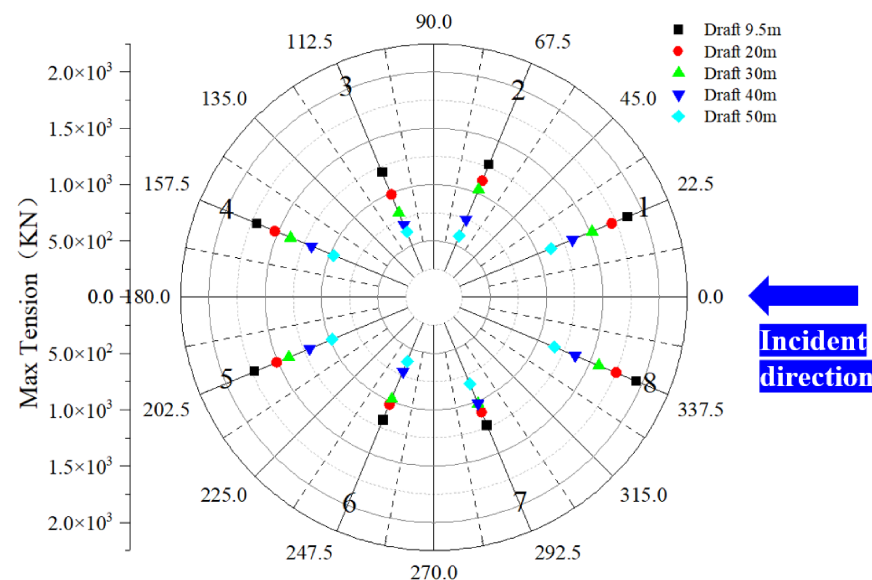
Figure 11. Mooring tension of Case 1 at 0^\circ incidence angle under different drafts.
