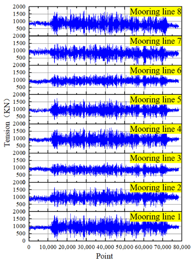
Figure 9. Mooring line tension curve.
