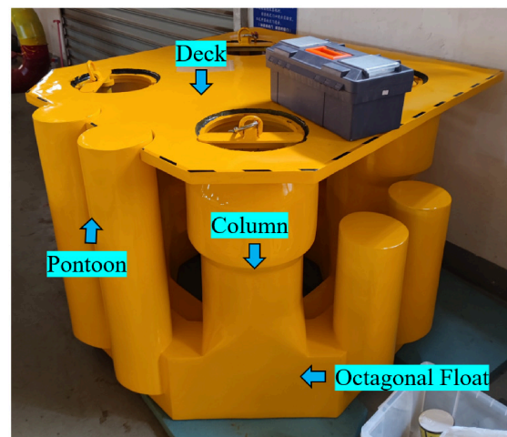
(b) OCTABUOY platform main structure model
