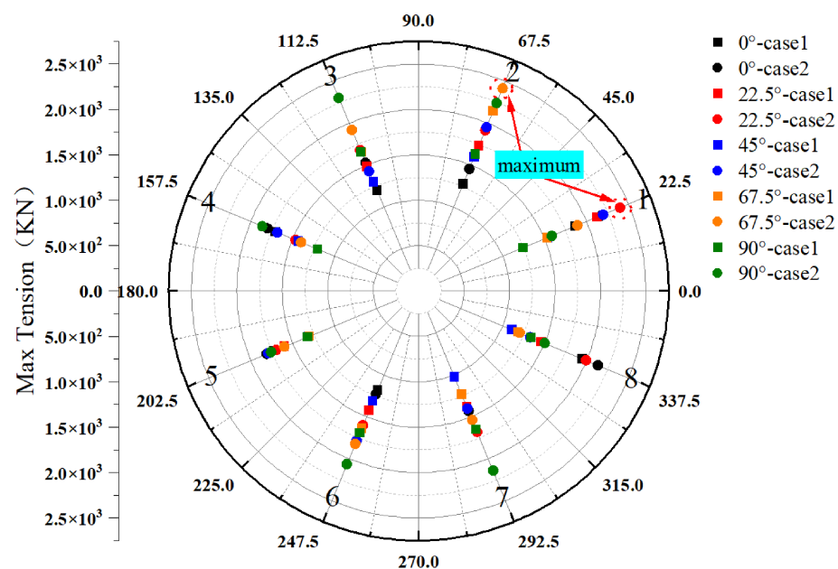
Figure 12. Maximum mooring tension calculation results.
