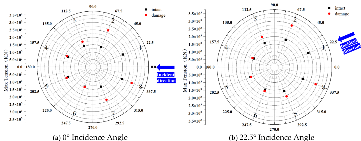
Figure 13. Mooring cable tension analysis.
