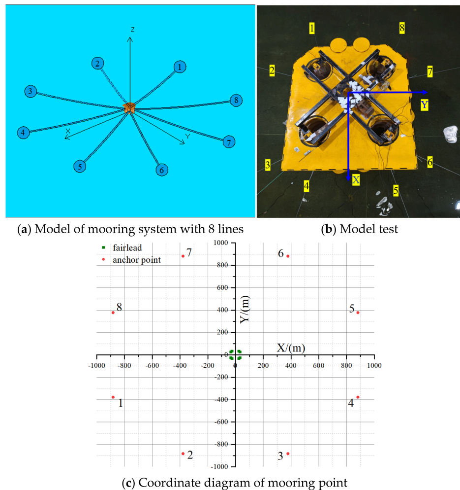
Figure 3. Arrangement of mooring system.
