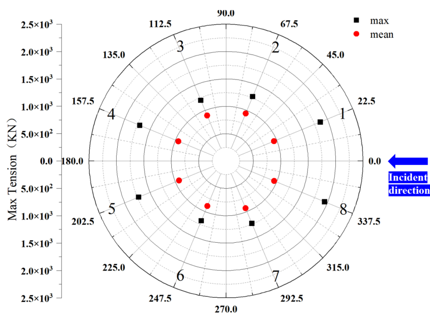
Figure 10. Mooring line tension comparison.
