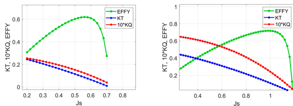
Figure 10. Open-water efficiency for pitch angles of service pitch angle +3^\circ (left) and +7^\circ (right).
