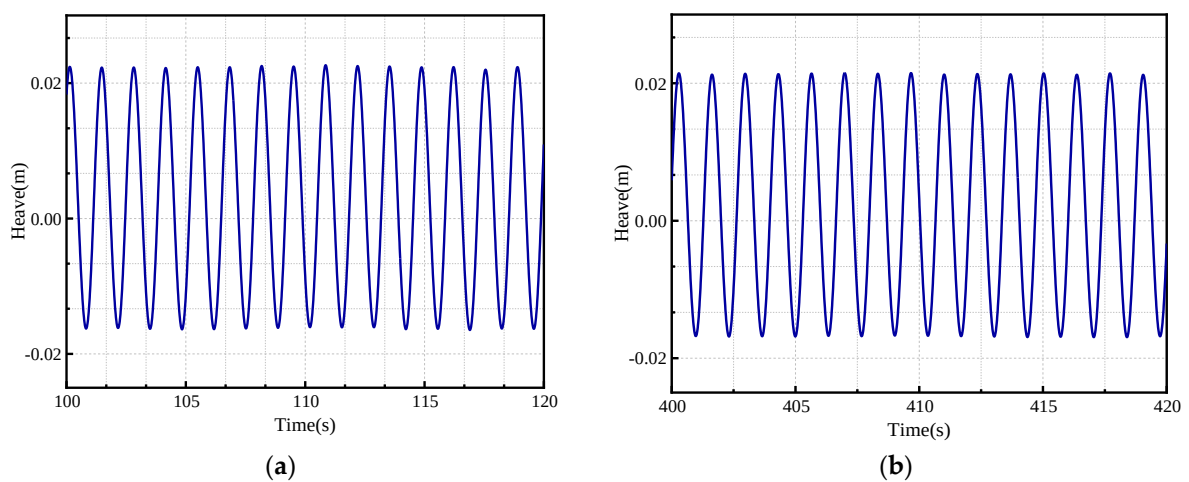
Figure 8. The time-history curve of heave motion. (a) 100–120 s local diagram, (b) 400–420 s local diagram.
