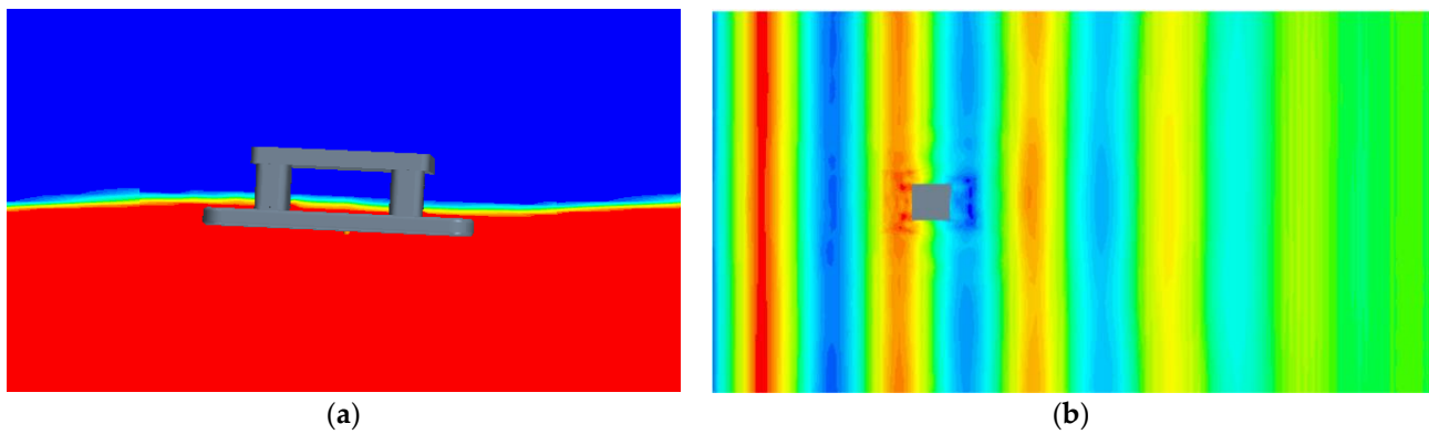
Figure 6. Numerical computation field. (a) Partial view from Y-axis perspective. (b) Overall view from Z-axis perspective.
