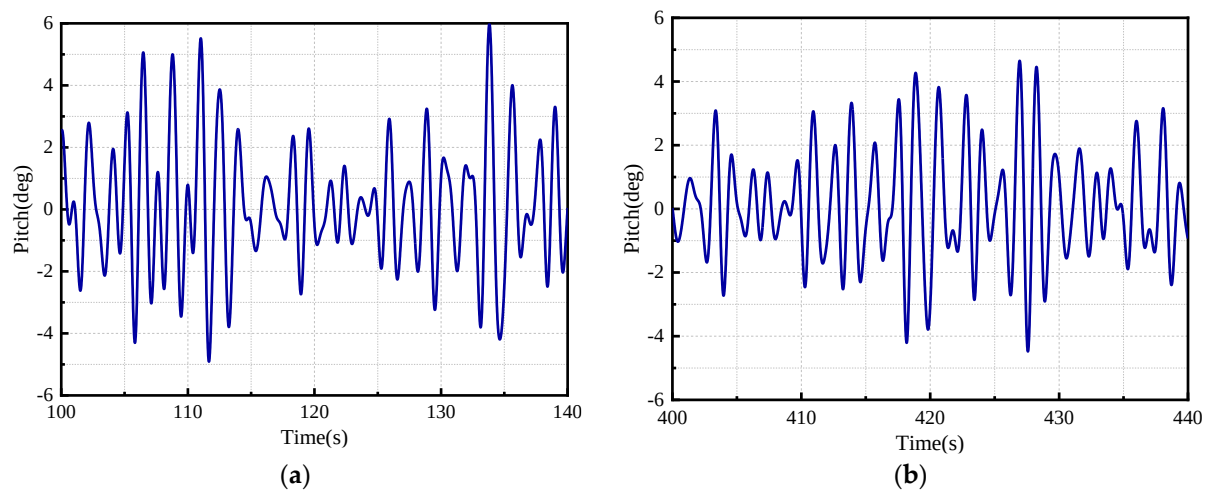
Figure 15. The time-history curve of pitch motion. (a) 100–140 s local diagram, (b) 400–440 s local diagram.
