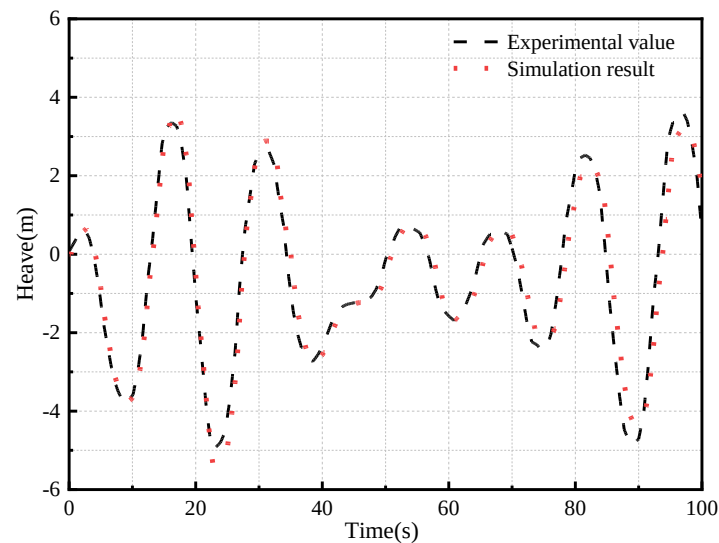
Figure 4. The comparison of heave motion between experimental value and simulation result.
