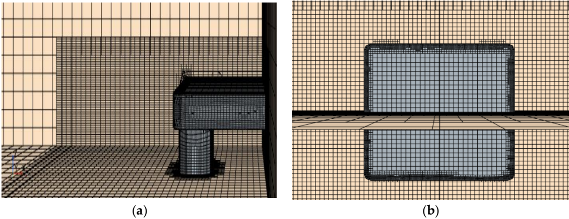
Figure 3. Grid division situation. (a) Y-axis direction. (b) Z-axis direction.
