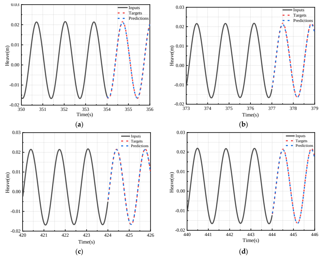
Figure 11. Heave test set single sample prediction result diagram. (a) 350–356s. (b) 373–379s (c) 420–426s (d) 440–446s.
