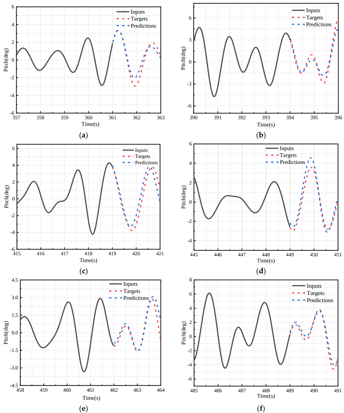
Figure 18. Pitch test set single sample prediction result diagram. (a) 357–363 s. (b) 390–396 s. (c) 415–421 s. (d) 445–451 s. (e) 458–464 s. (f) 485–491 s.
