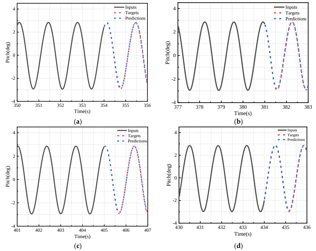
Figure 12. Pitch test set single sample prediction result diagram. (a) 350–356s. (b) 377–383s (c) 401–407s (d) 430–436s.
