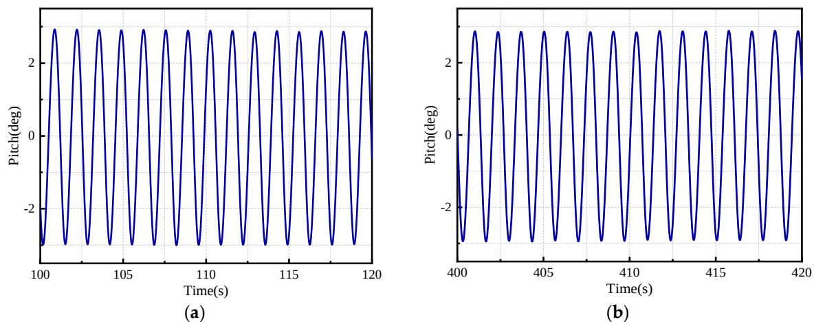
Figure 9. The time-history curve of pitch motion. (a) 100–120 s local diagram, (b) 400–420 s local diagram.
