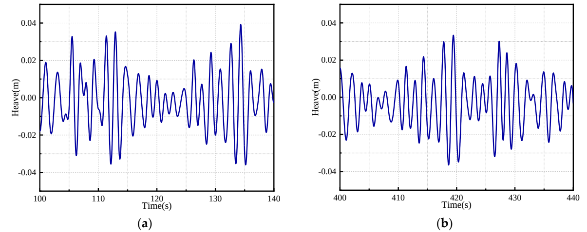
Figure 14. The time-history curve of heave motion. (a) 100–140 s local diagram, (b) 400–440 s local diagram.
