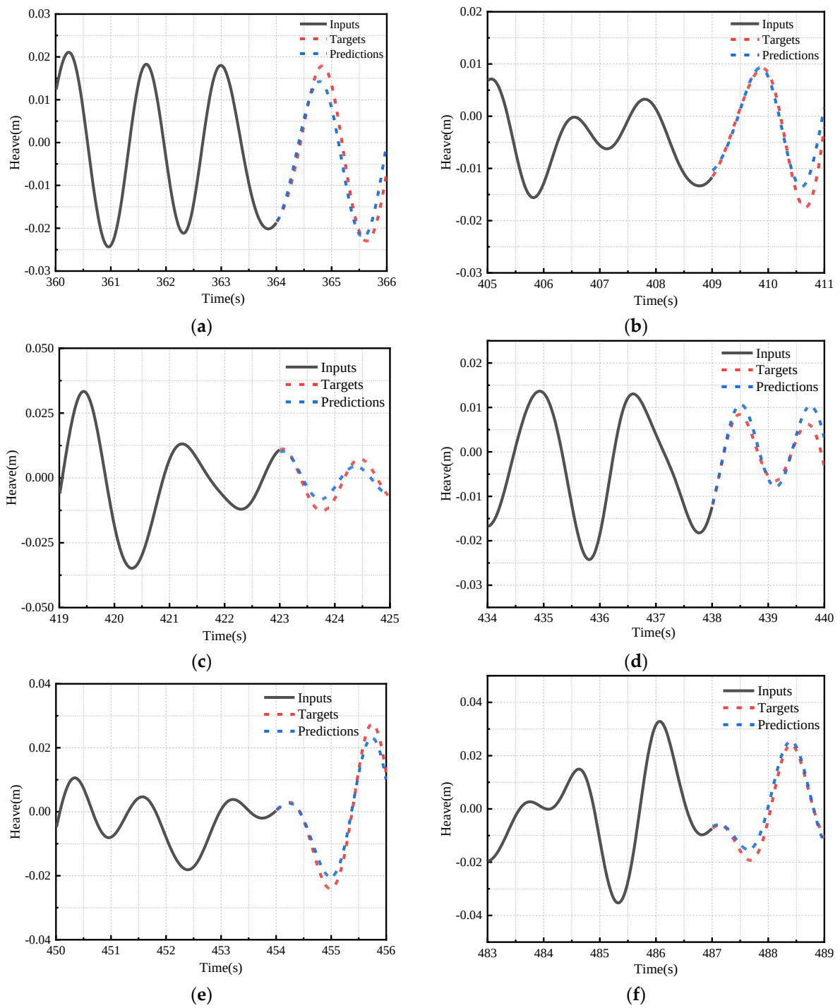
Figure 17. Heave test set single sample prediction result diagram. (a) 360–366 s. (b) 405–411 s (c) 419–425 s (d) 434–440 s (e) 450–456 s (f) 483–489 s.
