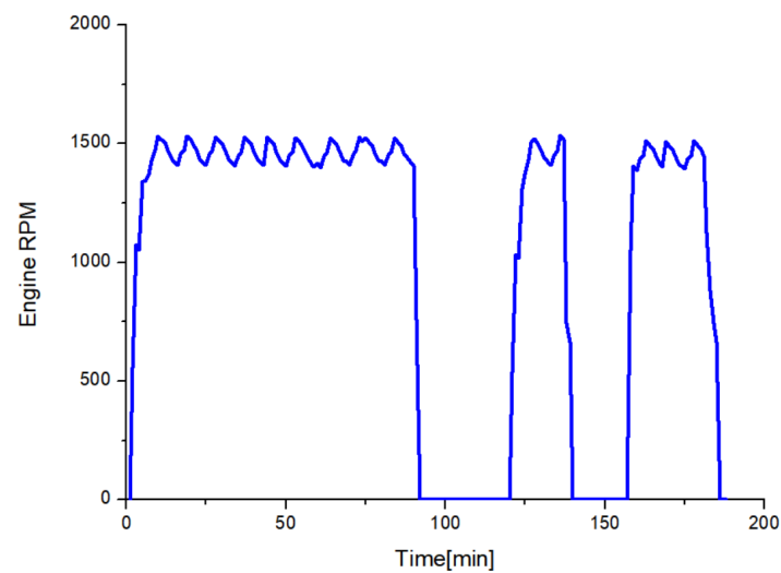
Figure 7. rpm of the reference fishing boat.
