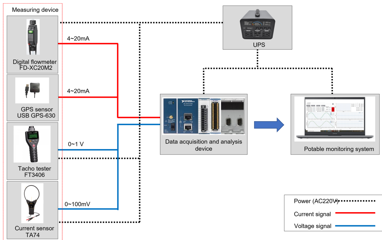
Figure 2. Configuration of data acquisition and analysis system.
