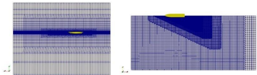
Figure 1. Mesh representation.
