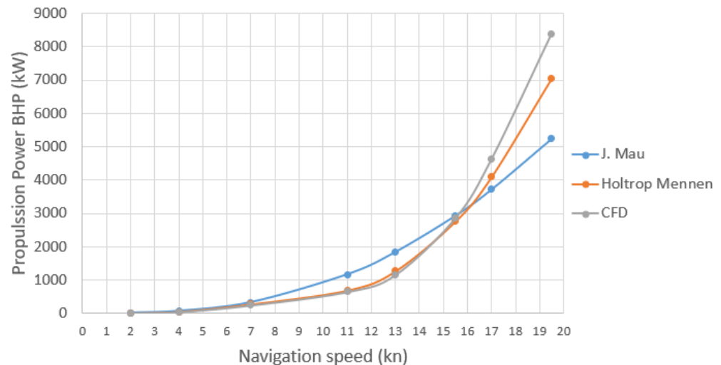
Figure 3. BHP requirement for different speeds according to the resistance estimation methods.
