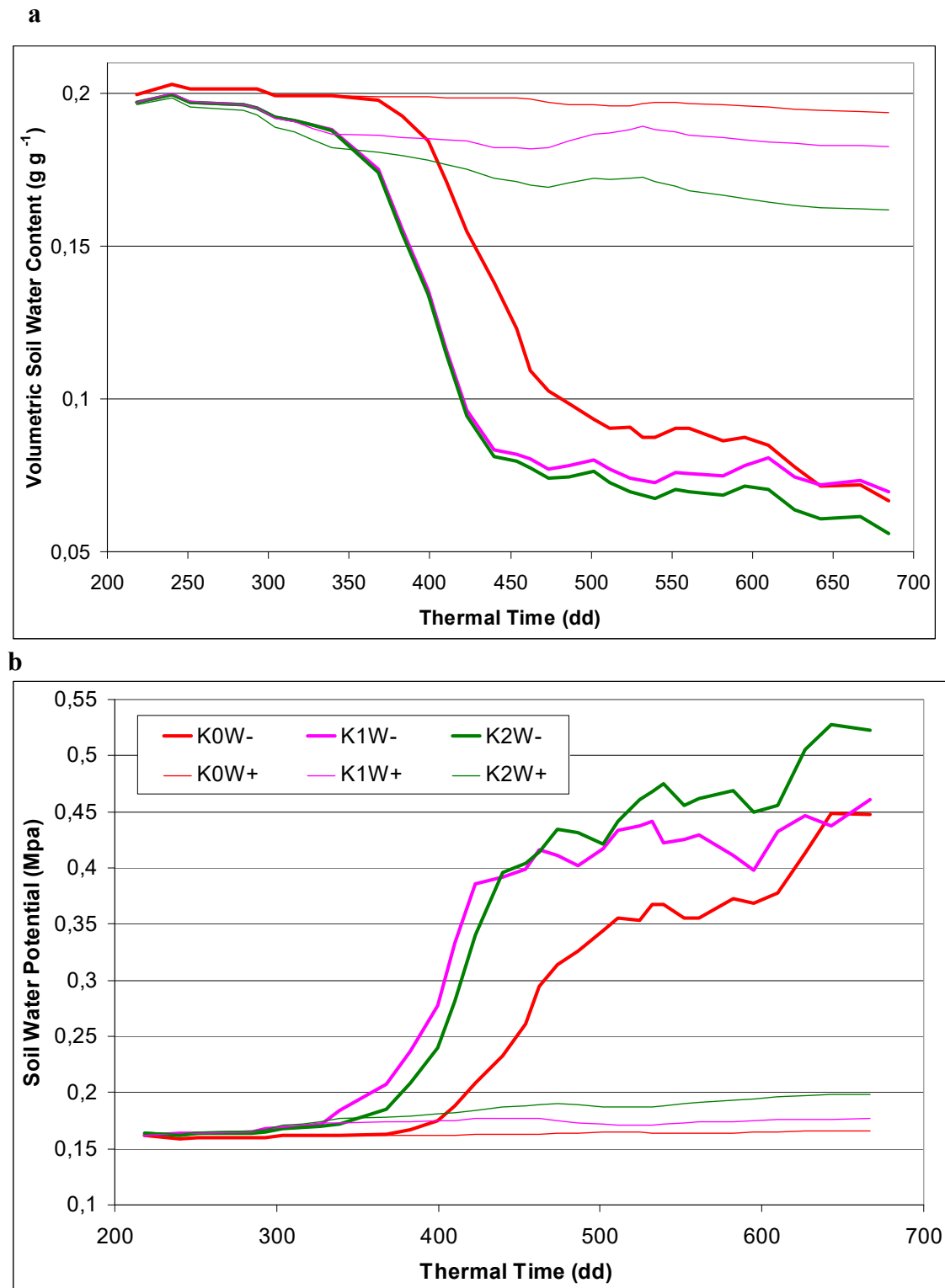
Figure S1: Evolution of a) the volumetric Soil Water Content and b) the corresponding soil water potential. The soil water content was obtained by weighing pots regularly (Equation 3). The soil water potential was obtained by pre-dawn water potentials measurements at the end of the experiment as well as by a relationship obtained between soil water content and soil water potential on a previous greenhouse-pot experiment using the same soil.
