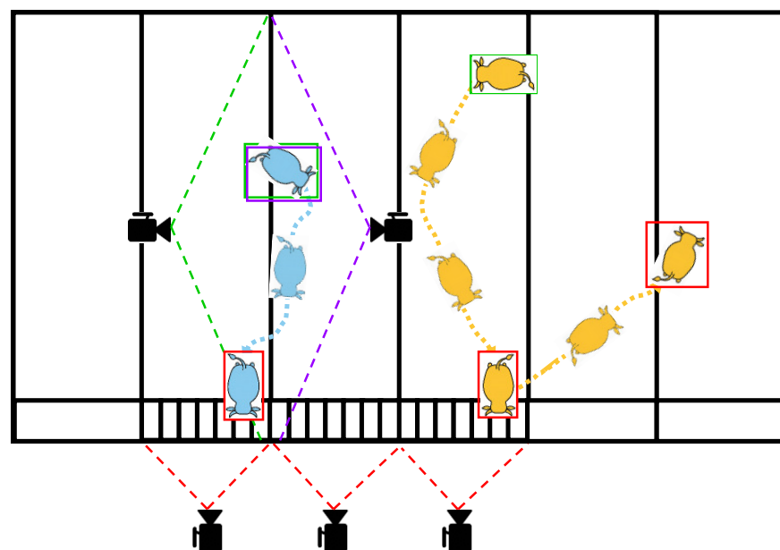
Figure 2. Schematic illustration of the multi-view trajectory association framework. The figure demonstrates the trajectory matching strategies across action–action cameras and across action–face cameras on a unified BEV map.
