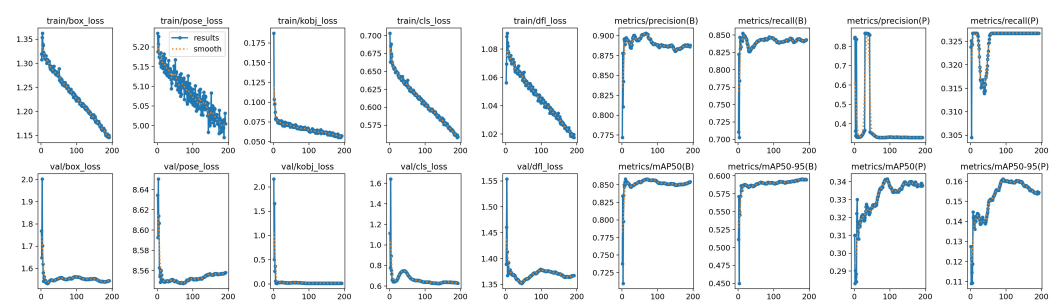
Figure 7. Training and validation curves of the detection and keypoint estimation model. ( Top ): Training losses and metrics. ( Bottom ): Validation losses and mAP scores across two tasks.
