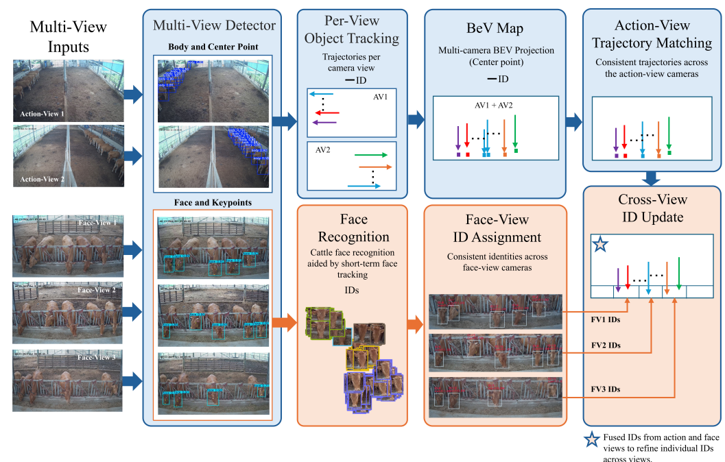
Figure 4. The workflow of the proposed cattle tracking system. The system first takes multi-view images as Inputs, which are processed by the detector to identify cattle in both action and face views. The Tracker generates temporal trajectories from action views, which are further projected onto a BEV map for spatial alignment. The Action-View Trajectory Matching module performs trajectory association across views. In parallel, the Face Recognition module extracts facial features and recognizes identities, then Face-View ID Assignment labels individual cattle. Finally, the Cross-View ID Update integrates trajectory and face information to maintain consistent identities across all views.
