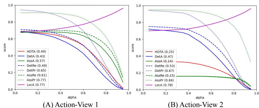
Figure 13. HOTA evaluation curves on two Action-View cameras. (A,B) show Detection, Association, and Localization Accuracy across different \alpha values for Action-View 1 and Action-View 2, respectively.
