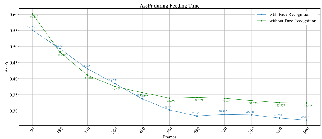
Figure 15. AssPr scores during the feeding period, highlighting the contribution of face recognition.
