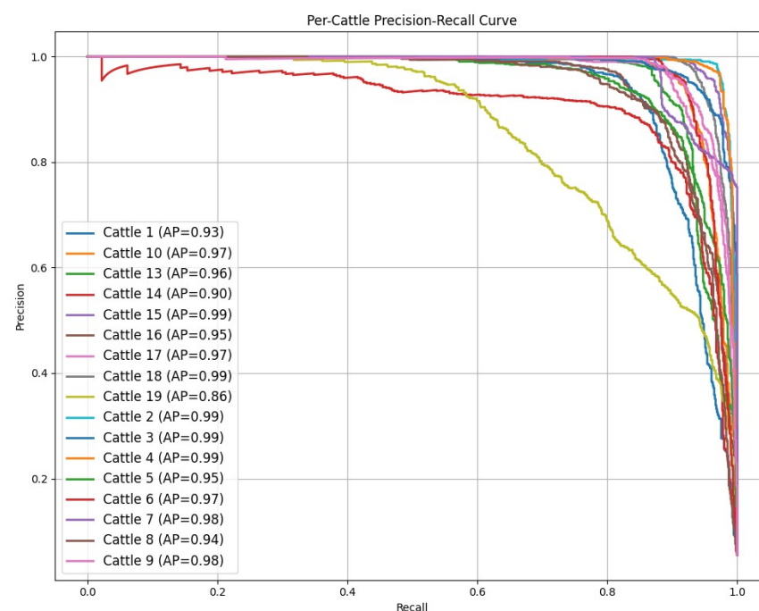
Figure 9. Precision–recall curves for individual cattle in face recognition. Each curve corresponds to one identity, with AP noted in the legend. The results show consistently high precision across most individuals.
