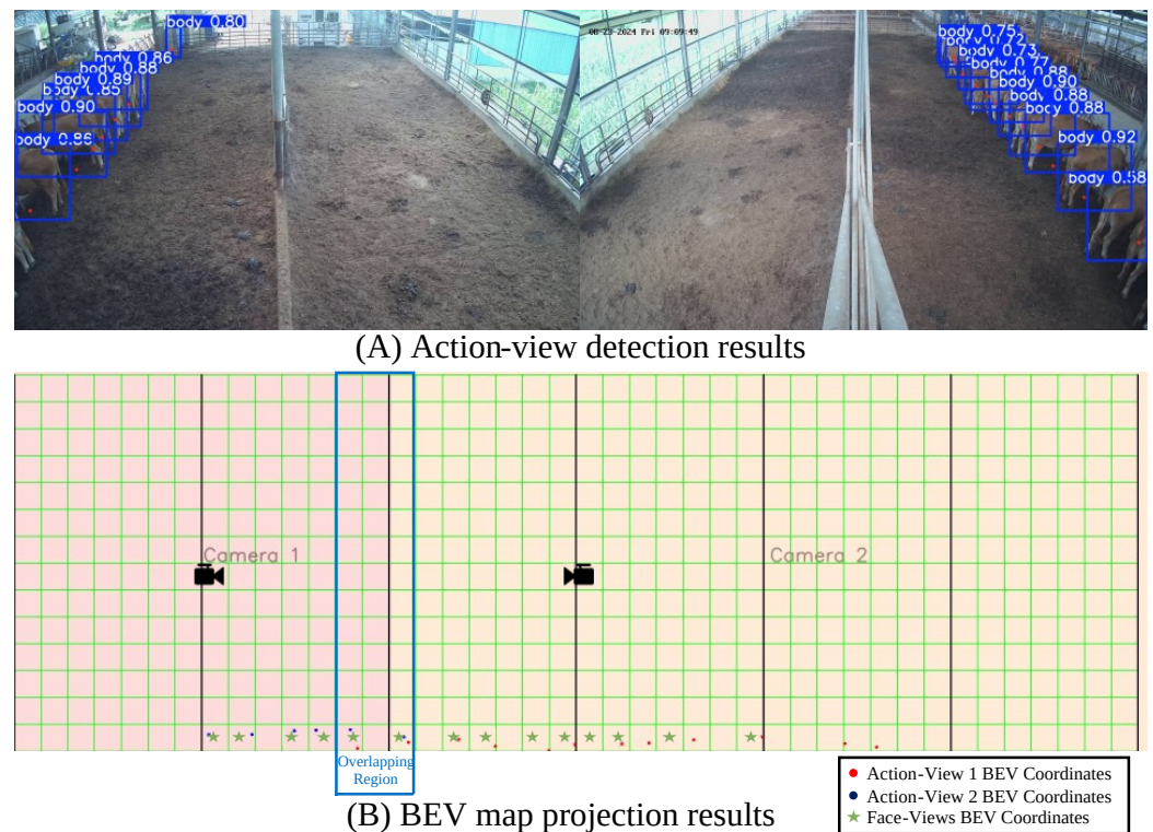
Figure 6. Body detection and BEV projection under grid mapping. The upper part shows detection results from Camera 1 and Camera 2, where bounding boxes are drawn for each detected cattle. The lower part illustrates the corresponding BEV projection of detected center points onto a grid-based spatial layout. Each dot represents a projected location of a detected instance.
