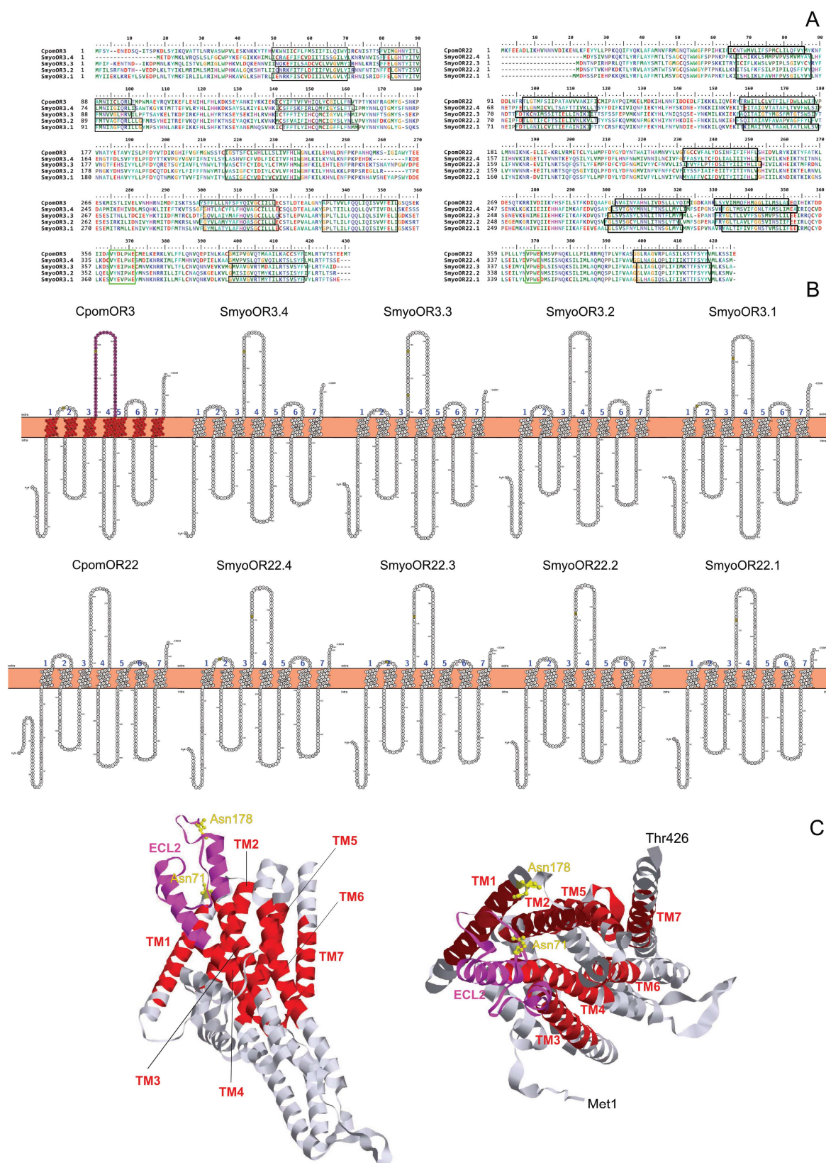
Figure 6. Polypeptide sequence and structural analysis. (A) polypeptide sequence alignment of the C. pomonella CpomOR3 (left) and CpomOR22 (right) with the respective S. myopaeformis subunits.
