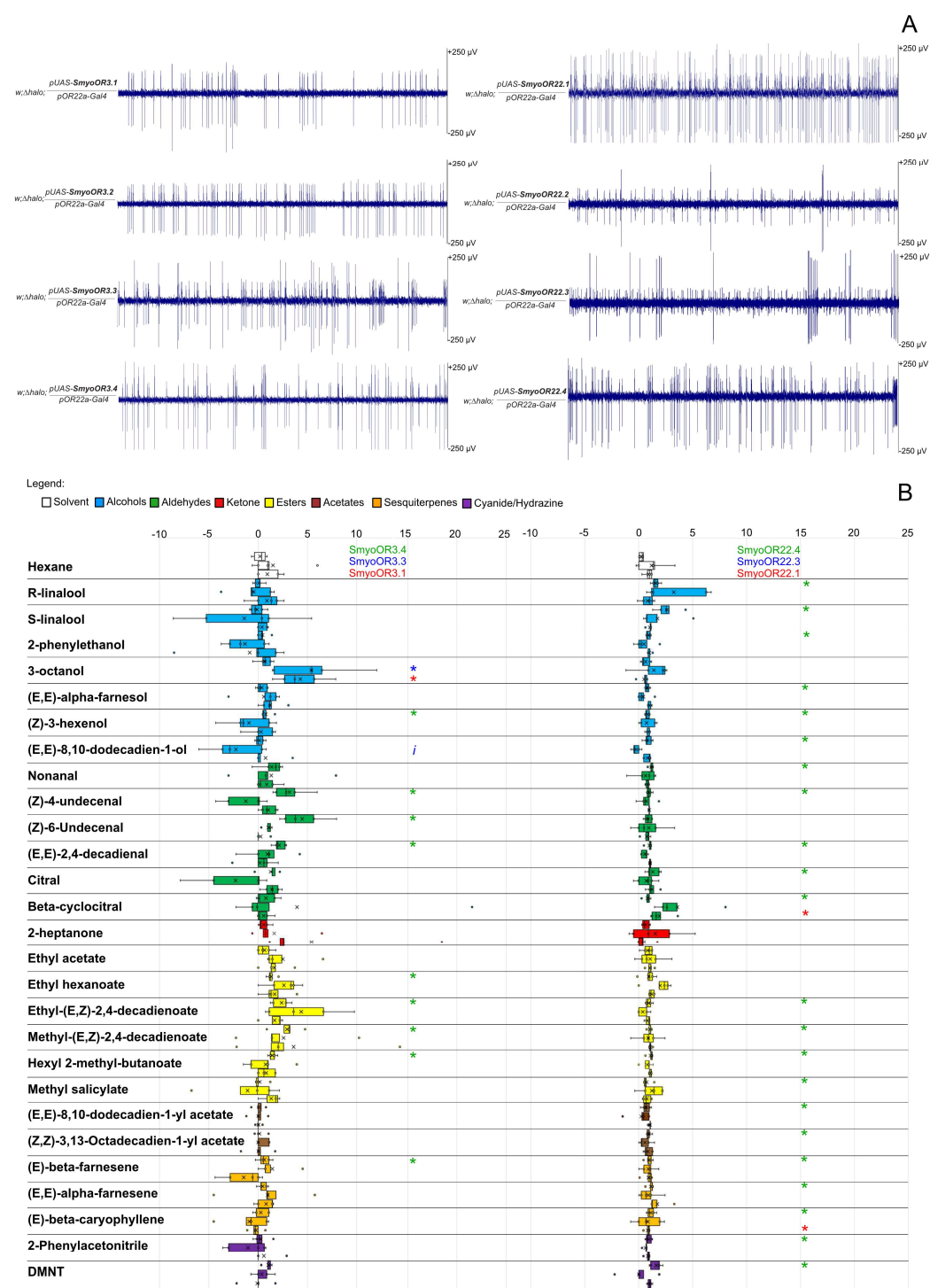
Figure 3. Functional expression of SmyoOR subunits. (A) Basic spiking of SmyoOR subunits. Note: expression of SmyoOR3.2 and SmyoOR22.2 unveiled absence of spiking. (B) Box-plot analysis of
