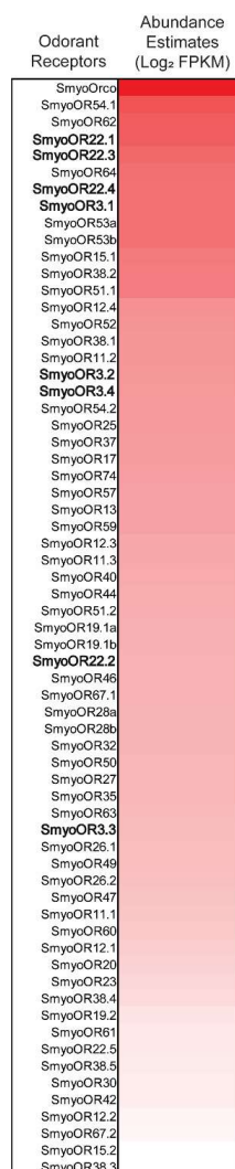
Figure 2. Heat plot of relative expression values for Synanthedon myopaeformis odorant receptors (ORs). Estimation of abundance values determined by read mapping. Receptors are sorted according to decreasing abundance: white and lighter pink colours indicate relatively lower expression, darker pink and red indicate relatively higher expression. Colour plots represent binary log of FPKM for each gene (See Supplementary Data File S6 for raw data). A larger bold font is used to indicate ORs functionally examined in this report. Range of values for male antenna: 0.44–7.46.
