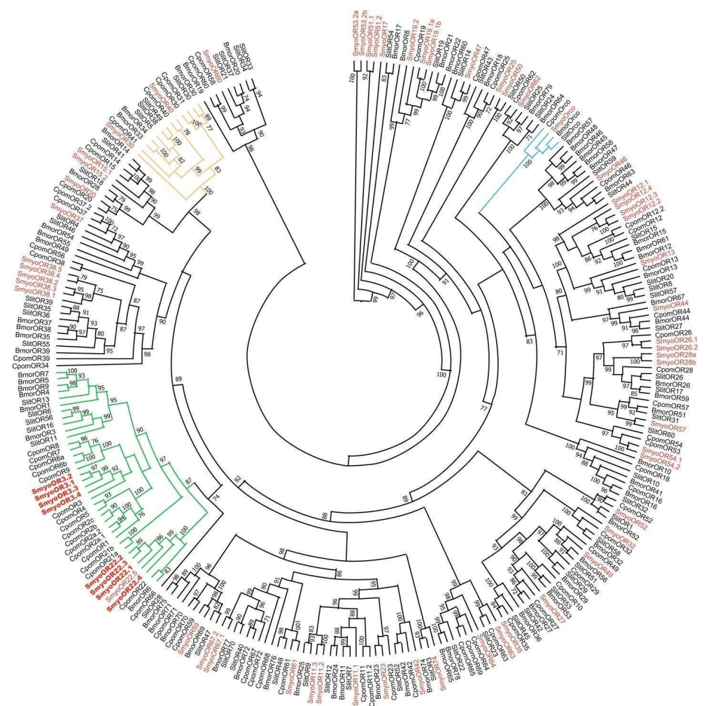
Figure 1. Maximum likelihood phylogenetic tree of candidate SmyoOR sequences with other lepidopteran OR sequences. Unrooted phylogenetic tree built using the online tool PhyML 3.0. Includes sequences from Bombyx mori (Bmor), Cydia pomonella (Cpom), and Spodoptera littoralis (Slit). Branches of the Orco clade are coloured light blue; branches of the lepidopteran canonical “Pheromone Receptor” clade are coloured green; branches of the expanded novel pheromone receptor clade are coloured orange; S. myopaeformis ORs are indicated with red font and those functionally studied in this report are marked with bold font. Node support was assessed with the Shimodaira–Hasegawa approximate likelihood ratio test (SH-aLRT); values greater than 0.7 are shown.
