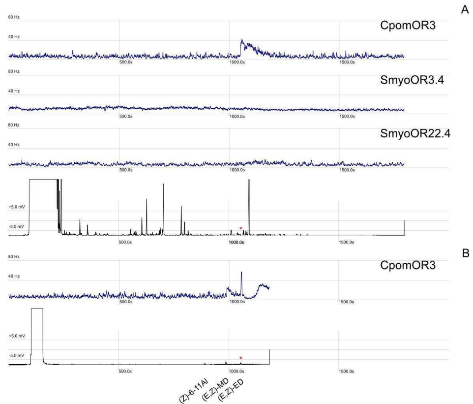
Figure 5. GC-SSR analysis of headspace. (A) Example from the headspace effects when testing the headspace Hoplomalus 562 from our previous study [29] on transgenic Drosophila expressing CpomOR3 (N = 11), SmyoOR3.4 (N = 3), and SmyoOR22.4 (N = 4). Red asterisk denotes the peak that possibly correlates with pear ester as in B. (B) Comparison with authentic samples testing the same CpomOR3 insect from A with the blend of (Z)-6-undecenal [Z6-11Al], methyl-E,Z-2,4 decadienoate [(E,Z)-MD], and ethyl-E,Z-2,4 decadienoate [(E,Z)-ED] 5.0 µg/µL. Below: the GC spectrum indicated peaks associated with 5.0 ng doses (GC 10 mV). Frequency plot (SSR 80 Hz) represents ab3A spikes per second, set with a Bin width of 100 ms seconds and a smooth filter line with 25 Taps. Note: both (E,Z)-MD and (E,Z)-ED enhance increment in the CpomOR3 spike frequency. Note: recordings from Figure 5 have been performed the same day (6 December 2019) using exactly the same headspace vial.
