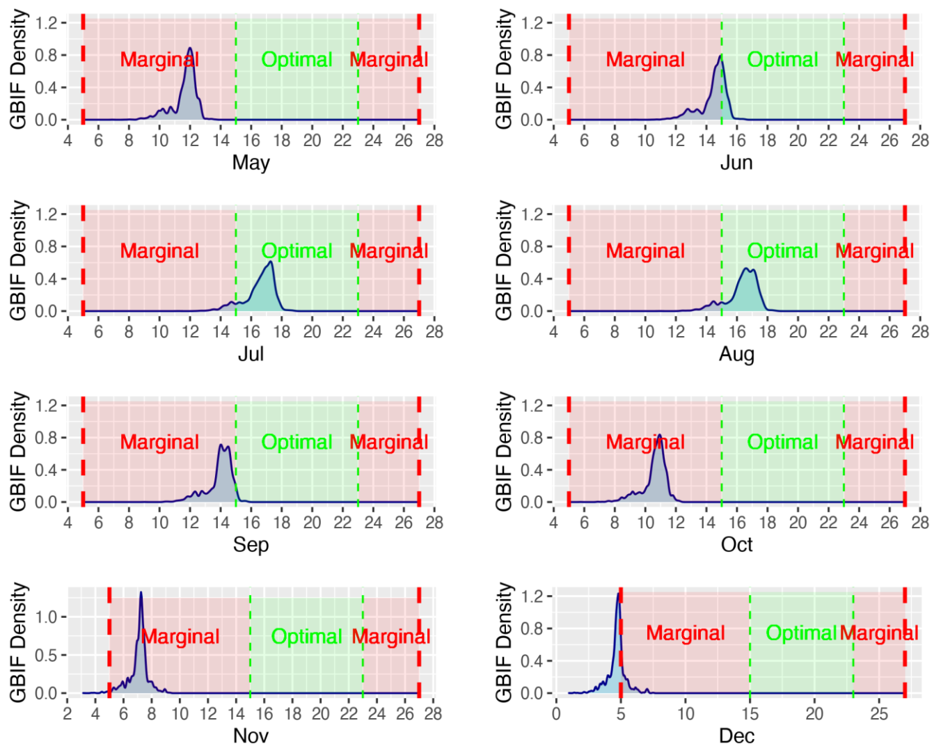
Figure A1. Seasonal suitability of wheat in the UK.
