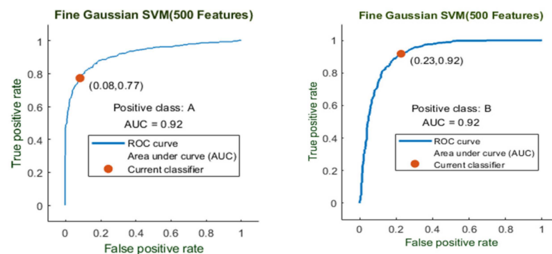
Figure 19. ROC curve for two classes A and B with 500 features and using 10-fold results.
