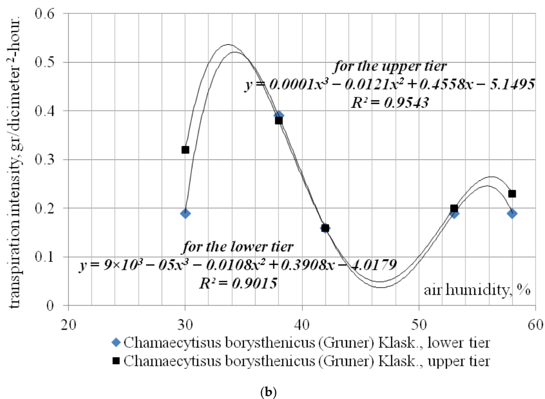
Figure 3. Change in transpiration intensity of Chamaecytisus borysthensis (Gruner) Klask. depending on changes in temperature (a) and humidity (b) of the air in the conditions of the dry steppe zone of Russia in sandy soils.
