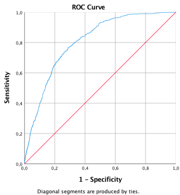
Figure S1. ROC Curve for hs-TnT for prediction of in-hospital mortality, AUC = 0.81.
