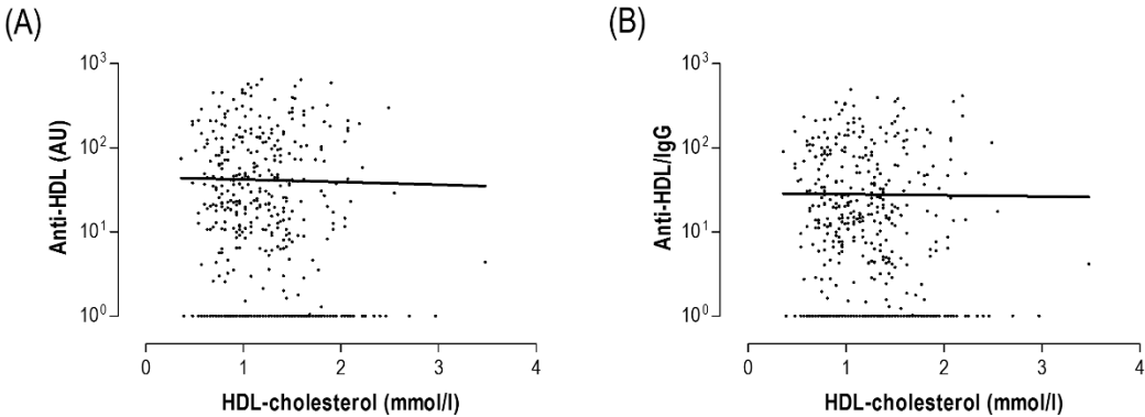
Supplementary Figure 1: Association between anti-HDL levels and circulating HDLc. The univariate association between anti-HDL measured as AU (A) or corrected by total IgG (B) and circulating HDL levels in AAA patients is shown.
