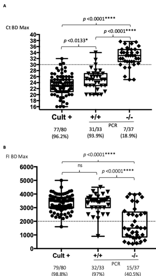
Figure 1. Stratification of the BD MAX TM results according to culture results and Campylobacter sp. detection by independent PCR formats (* p < 0.05 , and *** p < 0.001 , ns: non-significant). (A) Data analyzed according to the Ct values obtained on BD MAX TM ; (B) Data analyzed according to the fluorescence intensity (FI) obtained on BD MAX TM . Cult+: positive Campylobacter cases; +/-: culture negative cases positive by two independent PCRs; -/-: double-negative cases. The dotted lines correspond to the proposed cut-off for Ct or FI values.
