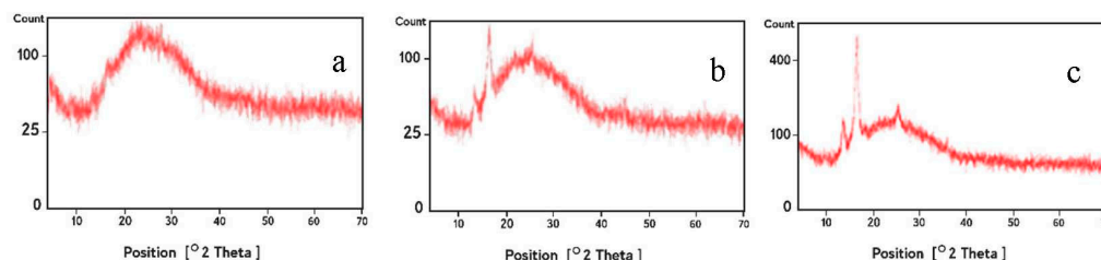
Figure 4. XRD analysis of (a) crosslinked gelatin nanofibers scaffolds before plasma treatment, (b) nanofibers after argon plasma treatment and (c) nanofibers after argon–oxygen plasma treatment.
