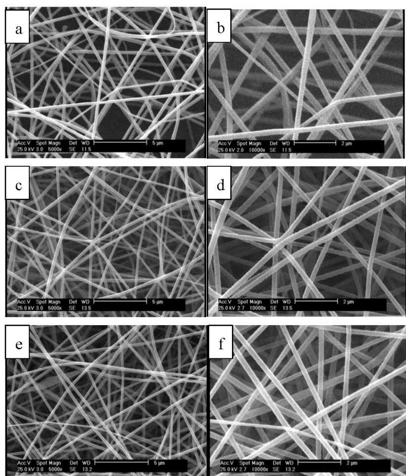
Figure 1. SEM images of: (a) nanofibers before plasma treatment at \times 5000 , (b) nanofibers before plasma treatment at \times 10,000 , (c) nanofibers after treatment with argon plasma at \times 5000 , (d) nanofibers after treatment with argon plasma at \times 10,000 , (e) nanofibers after treatment with argon–oxygen plasma at \times 5000 and (f) nanofibers after treatment with argon–oxygen plasma at \times 10,000 .
