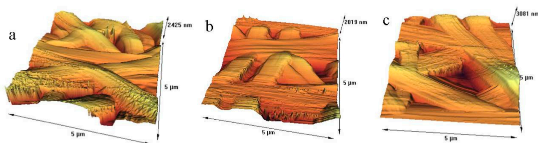
Figure 2. Atomic force microscopy (AFM) images of: (a) nanofibers before plasma treatment, (b) nanofibers after treatment with argon plasma and (c) nanofibers after treatment with argon–oxygen plasma.
