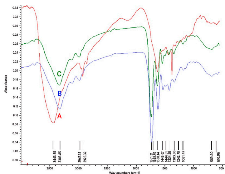
Figure 3. The attenuated total reflection Fourier transform infrared (ATR-FTIR) spectra of (A) crosslinked gelatin nanofibers before plasma treatment, (B) argon plasma treated nanofibers and (C) argon–oxygen plasma treated nanofibers.
