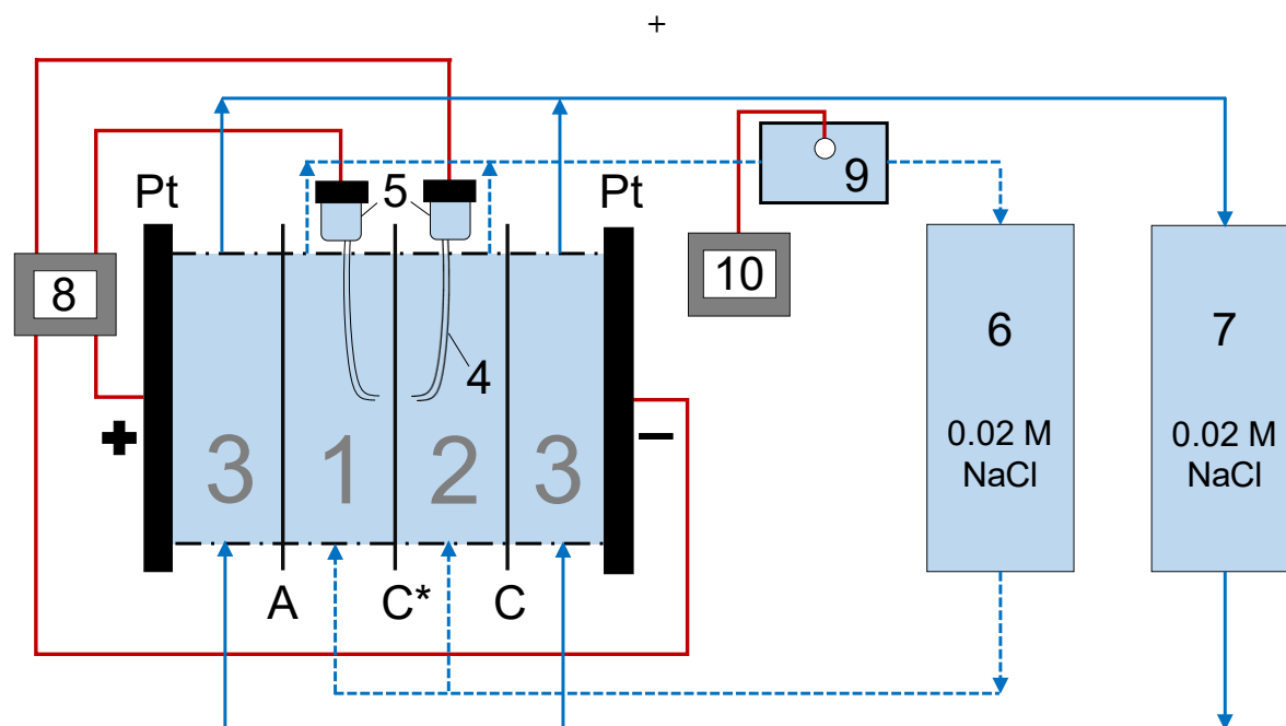
1—desalination chamber, 2—auxiliary chamber, 3—electrode chambers, 4—capillaries, 5—Luggin electrodes, 6—tank gathering solution from desalination and auxiliary chambers, 7—tank gathering solution from electrode chambers, 8—voltmeter and power supply, 9—interstitial tank in desalination track holding glass electrode and conductivity cell, 10—pH meter and conductometer. C* is a studied membrane, C and A are auxiliary cation exchange and anion exchange membranes, respectively.
