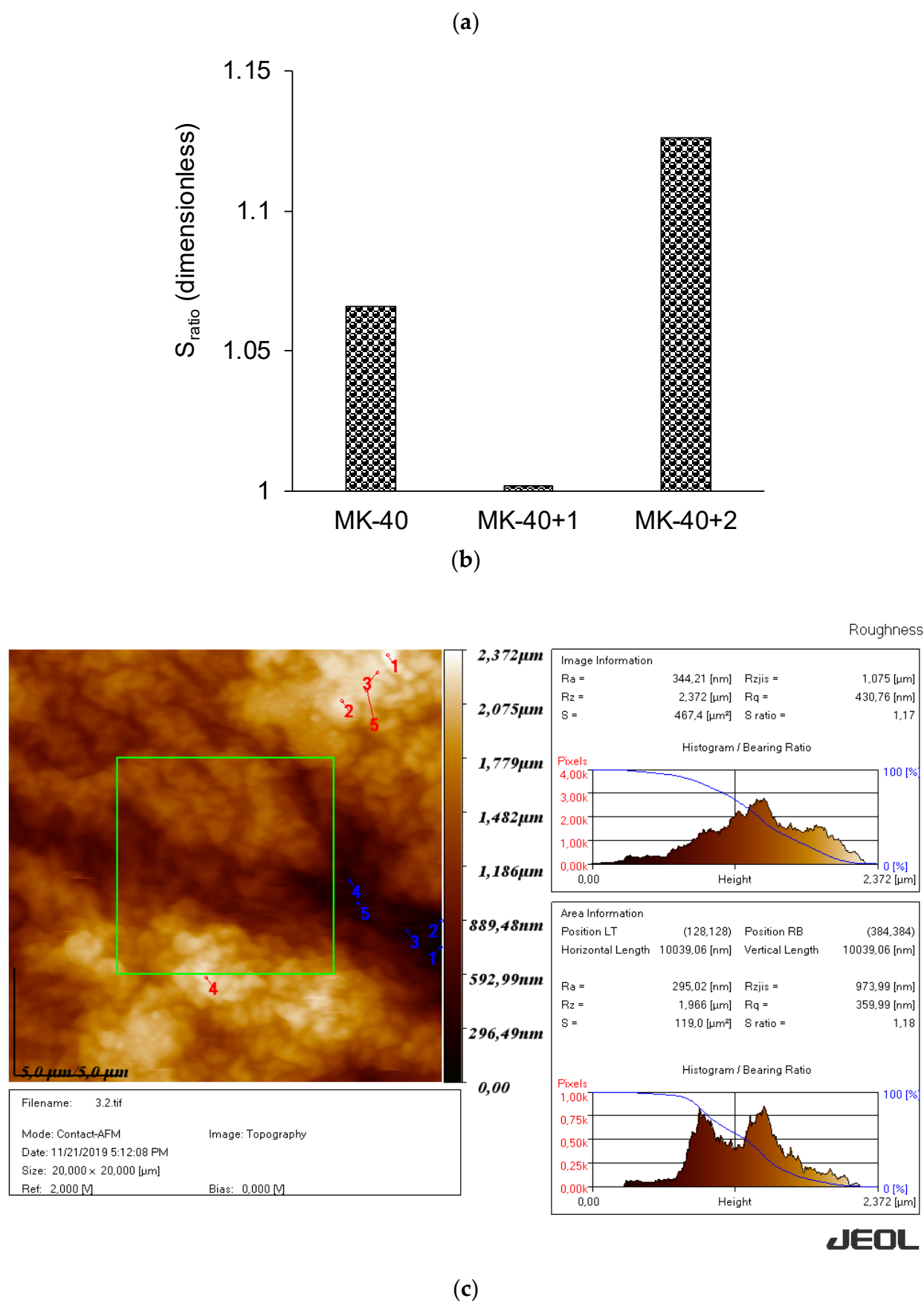
Figure 7. The roughness profile, R_a (a), and the ratio of the true area of the membrane to the ideal (absolutely flat) area, S_{ratio} (b) roughness parameters of the membranes, determined using atomic force microscopy, and an example of the obtained visualization of surface profile of the MK-40+2 membrane (c). Other profiles are given in the Supplementary Materials.
