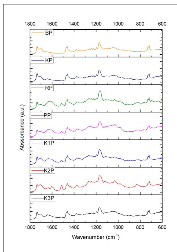
Figure 3. Average FTIR ATR spectrum of investigated propolis collected from five Adriatic Sea islands (Krk, Rab, Pag, Biševo and Korčula)—fingerprint region (1800–600 \text{cm}^{-1} ) emphasizing the most significant spectral variations.
