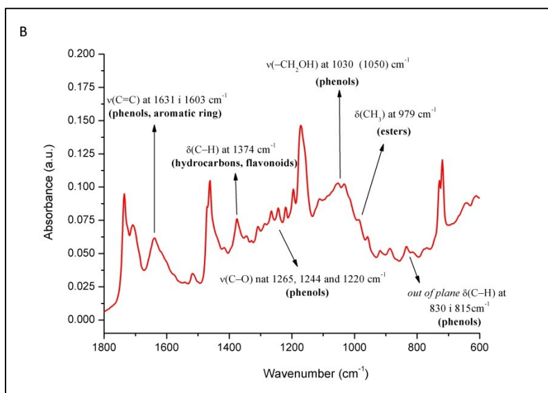
Figure 1. Characteristic FTIR-ATR spectrum of raw propolis (average K3 sample) with assigned underlying molecular vibrations: spectral region from 3800 to 500 \text{cm}^{-1} (A); fingerprint region 1800–600 \text{cm}^{-1} (B).
