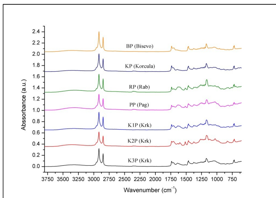
Figure 2. Average FTIR ATR spectrum of investigated propolis collected from five Adriatic Sea islands (Krk, Rab, Pag, Biševo and Korčula).
