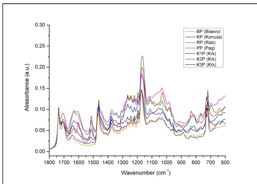
Figure 4. Overlaid average FTIR ATR spectrum of investigated propolis collected from five Adriatic Sea islands (Krk, Rab, Pag, Biševo and Korčula)—fingerprint region (1800–600 \text{cm}^{-1} ) emphasizing comparative spectral variations.
