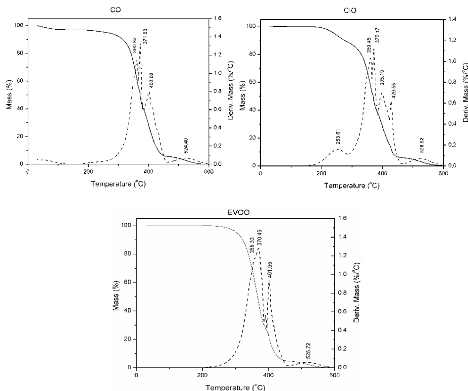
Figure 2. Mass Loss-Derivate (TG/DTG) thermograms of Colliguaya integerrima (CIO), Cynara cardunculus (CO), and extra-virgin olive (EVOO) oils.
