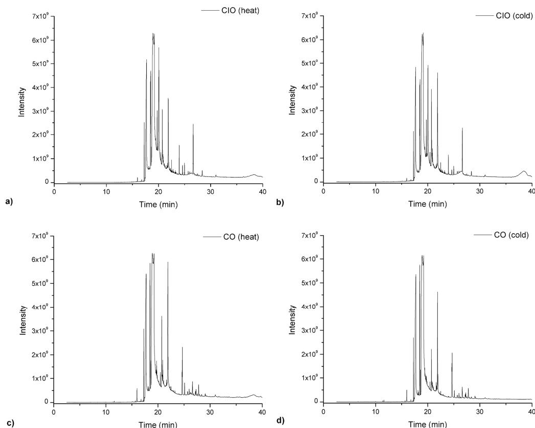
Figure 6. GC–MS chromatogram of CIO and CO after (a,b) and before (c,d) heating process, respectively.
