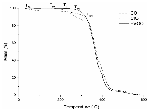
Figure 3. TG curve comparisons for the three different oils showing the selected temperatures corresponding to the degradation of Colliguaya integerrima (CIO), Cynara cardunculus (CO), and extra-virgin olive (EVOO) oils.
