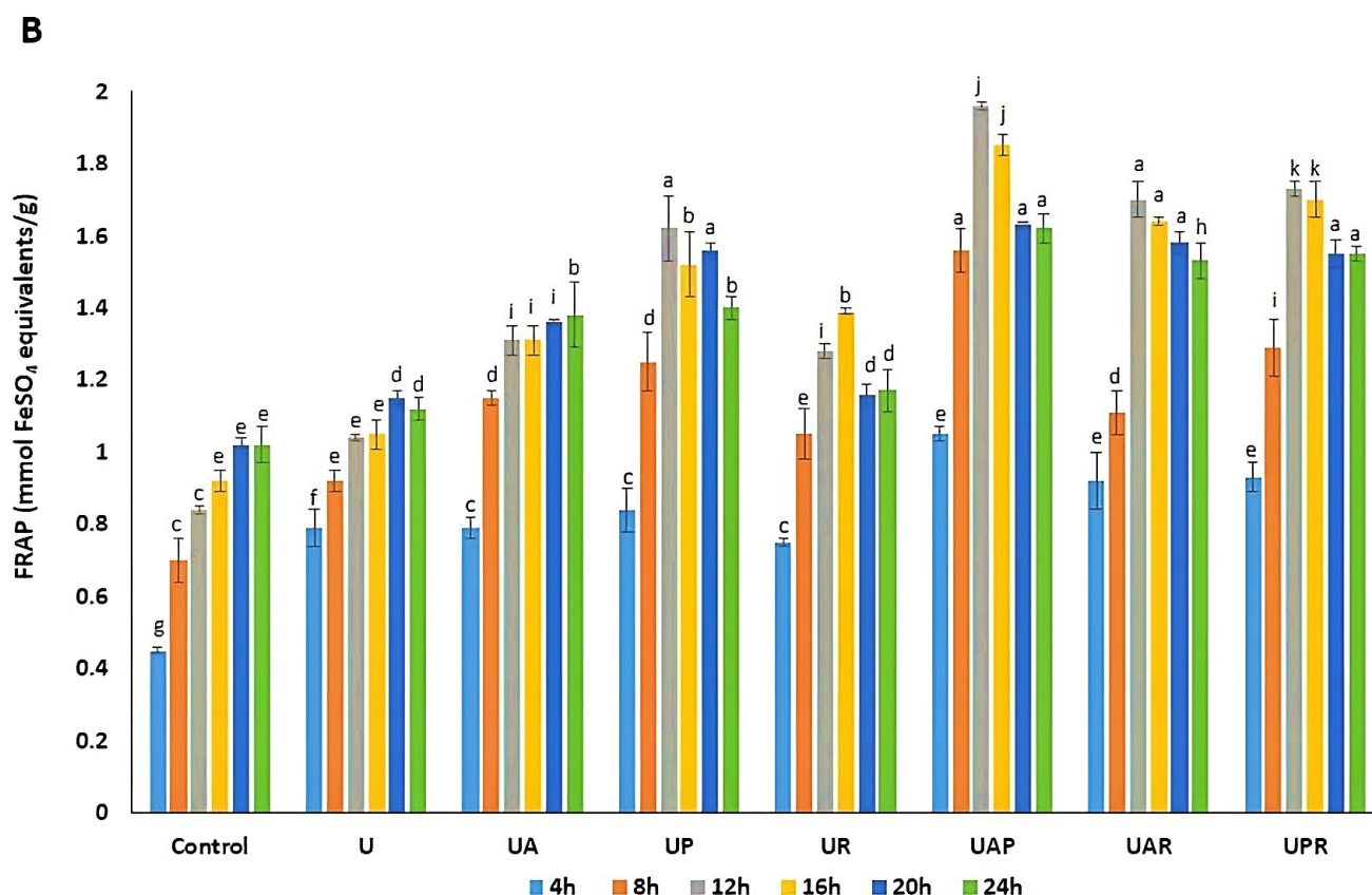
Figure 4. FRAP analysis of the (A) unfermented control, ultrasound-treated sample (U), and fermented E. amoenum using (A ( L. acidophilus ); P ( L. plantarum ); R ( L. reuteri ); AP ( L. acidophilus — L. plantarum ); AR ( L. acidophilus — L. reuteri ); PR ( L. plantarum — L. reuteri )); (B) unfermented control, ultrasound-treated sample (U), and ultrasound-assisted fermented E. amoenum (UA (Ultrasound-assisted L. acidophilus ); UP (Ultrasound-assisted L. plantarum ); UR (Ultrasound-assisted L. reuteri ); UAP (Ultrasound-assisted L. acidophilus — L. plantarum ); UAR (Ultrasound-assisted L. acidophilus — L. reuteri ); UPR (Ultrasound-assisted L. plantarum — L. reuteri )). Mean values \pm standard deviations are reported ( n = 3 ). In each graph, the same letter indicates not statistically different values ( p > 0.05 among values with same letter and p < 0.05 versus values with different letters).
