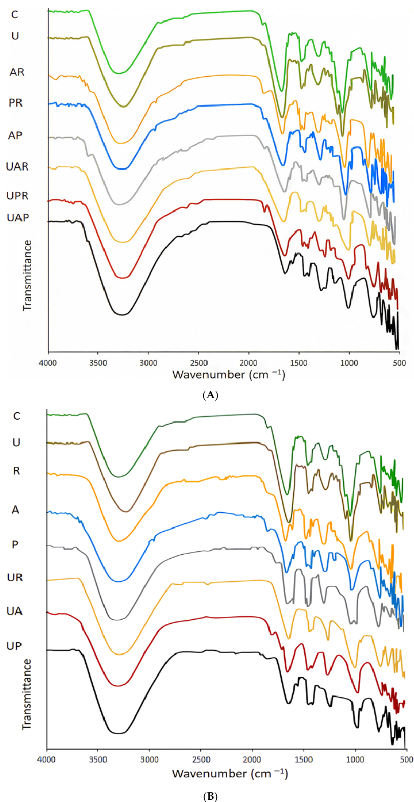
Figure 6. (A) FTIR spectra of the unfermented control E. amoenum sample (C), the ultrasound-treated sample (U), the mixed culture fermented samples ( L. acidophilus — L. reuteri (AR), L. plantarum — L. reuteri (PR), and L. acidophilus — L. plantarum (AP)), and the ultrasound-assisted mixed culture fermented samples ( L. acidophilus — L. reuteri (UAR), L. plantarum — L. reuteri (UPR), and L. acidophilus — L. plantarum (UAP)). (B) Spectra of the control unfermented E. amoenum sample (C); the ultrasound-treated sample (U); the single culture fermented samples ( L. acidophilus (A), L. reuteri (R), and L. plantarum (P)); and the ultrasound-assisted single culture fermented samples ( L. acidophilus (UA), L. reuteri (UR), and L. plantarum (UP)).
