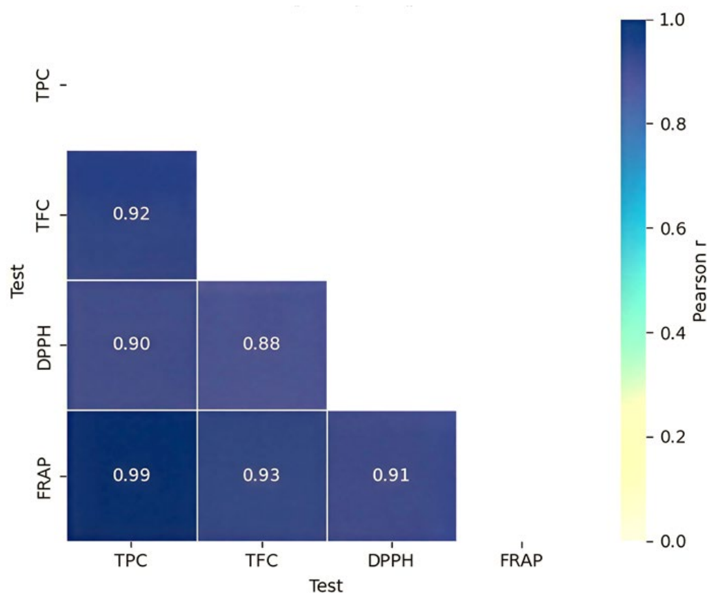
Figure 5. Correlation between TPC, TFC, and antioxidant activities (DPPH and FRAP).
