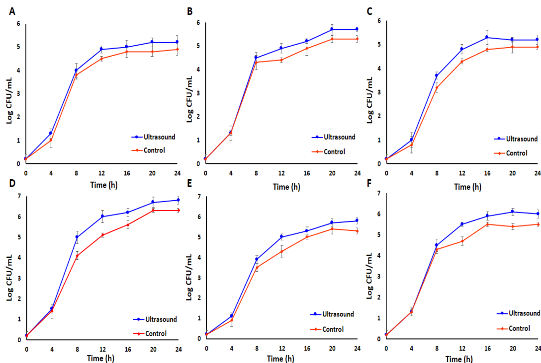
Figure 2. The effect of ultrasound treatment on LAB bacterial growth rate during the fermentation of E. amoenum at 37 °C for 24 h in single ( L. acidophilus (A), L. plantarum (B), L. reuteri (C)), and mixed ( L. acidophilus — L. plantarum (D), L. acidophilus — L. reuteri (E), and L. plantarum — L. reuteri (F)) cultures, compared to fermented control samples without ultrasound exposure.
