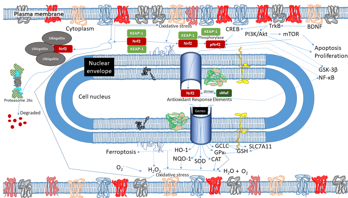
Figure 2. Simplified depiction of the mechanism of action of Nrf2 and the pathways it interacts with. Arrows, activation; broken lines with rhomboid ending, inhibition. Abbreviations. Akt, Protein kinase B; BDNF, brain-derived neurotrophic factor; CREB, cyclic AMP responsive element binding protein; GCLC, Glutamate-cysteine ligase; GPx, glutathione peroxidase; GSH, glutathione; GSK-3 \beta , glycogen synthase kinase 3-beta; HO-1, haem oxygenase 1; mTOR, mammalian target of rapamycin; NF- \kappa B, nuclear factor kappa B; NQO-1, NAD(P)H quinone dehydrogenase 1; PI3K, phosphatidylinositol-3-kinase; SLC7A11, Solute Carrier Family 7 Member 11 (cystine/glutamate transporter); sMAF, small musculoaponeurotic fibrosarcoma proteins; SOD, superoxide dismutase; TrkB, tropomyosin receptor kinase B.
