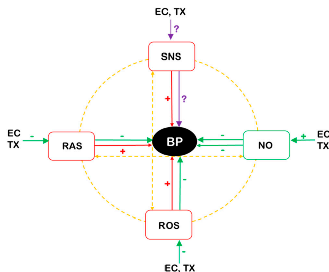
Figure 1. Scheme of interactions among the main blood pressure regulatory systems and reactive oxygen species. The SNS, RAS, ROS, and NO all participate in blood pressure regulation and interact with each other (orange lines). EC and TX were shown possess antioxidant properties and to reduce ROS. EC and TX also inhibit the RAS and elevate NO production (green lines). The SNS, RAS, and elevated ROS are known to elevate blood pressure (red lines). The effects of EC and TX directly on the SNS are unclear. Abbreviations: BP, blood pressure; EC, (–)-epicatechin; NO, nitric oxide; ROS, reactive oxygen species; SNS, sympathetic nervous system; RAS, renin–angiotensin system; TX, (+)-taxifolin, (–)-taxifolin or their racemic mixture.
