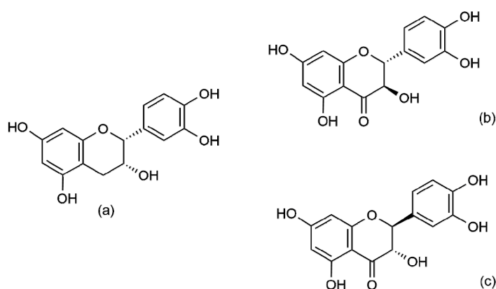
Figure 2. Structural formulas of (–)-epicatechin (a), (+)-taxifolin (b), and (–)-taxifolin (c).
