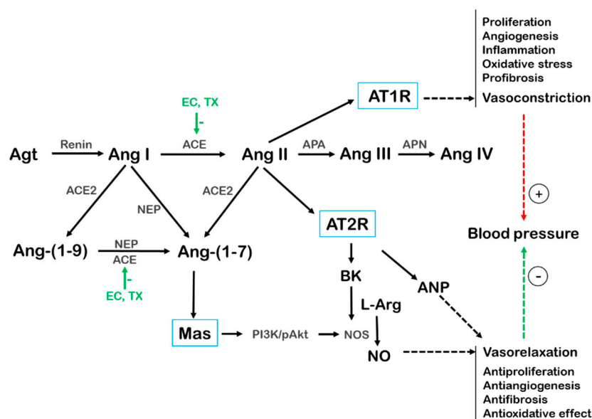
Figure 4. A brief, although not exhaustive, scheme of the renin–angiotensin system. Abbreviations: ACE, angiotensin converting enzyme; Agt, angiotensinogen; Ang, angiotensin; ANP, atrial natriuretic peptide; APA, aminopeptidase A; APN, aminopeptidase N; AT1R, angiotensin II type 1 receptor; AT2R, angiotensin II type 2 receptor; BK, bradykinin; EC, (–)-epicatechin; L-Arg, L-arginine; Mas, Mas receptor; NEP, neutral endopeptidase, NO, nitric oxide; NOS, nitric oxide synthase; PI3/Akt, phosphatidylinositol 3-kinase/kinase B; TX, (+)-taxifolin, (–)-taxifolin or their racemic mixture.
