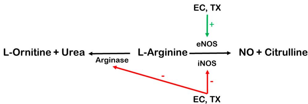
Figure 3. The EC- and TX-induced beneficial mechanisms involved in NO production. The green arrow indicates stimulation of the enzyme, which leads to the augmentation of NO production by eNOS. The red arrows indicate the EC- and TX-induced inhibition of the enzymes, leading to downregulation of iNOS in injured tissue and the inhibition of arginase. Abbreviations: EC, (–)-epicatechin; eNOS, endothelial nitric oxide synthase; NO, nitric oxide; TX, (+)-taxifolin, (–)-taxifolin or their racemic mixture.
